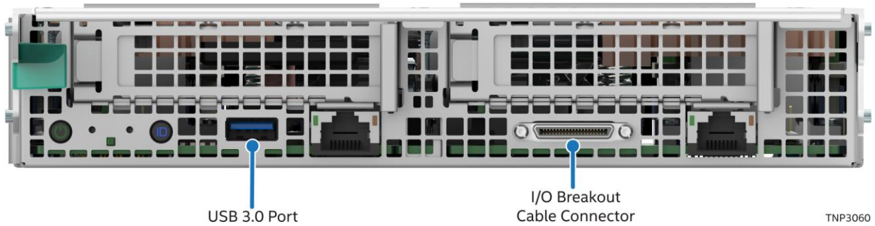
Figure 77. USB Port Location - 1U Compute Module
