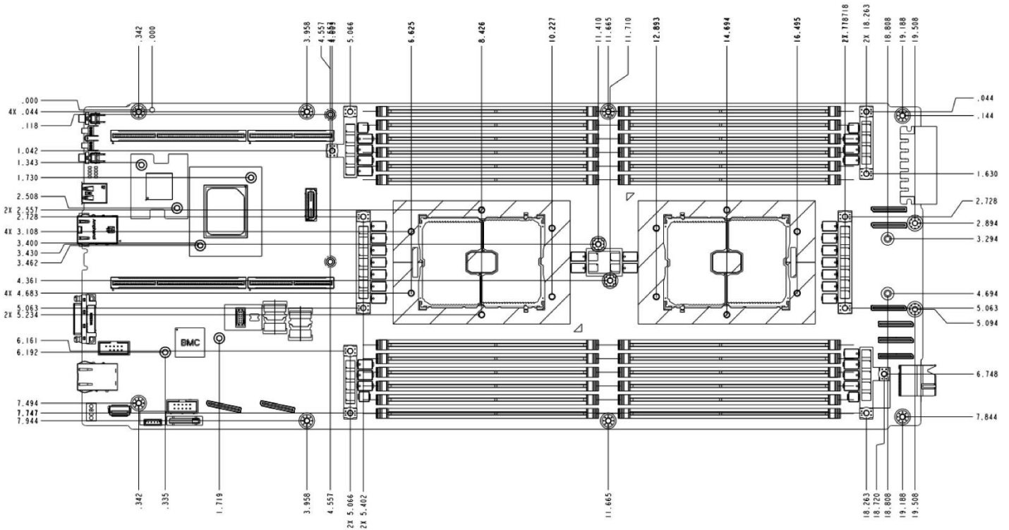
Figure 119. Intel® Server Board D50TNP1SB Components Position
