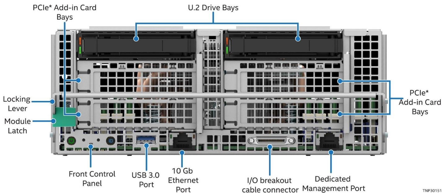
Figure 21. 2U Management Module Front Panel Features
