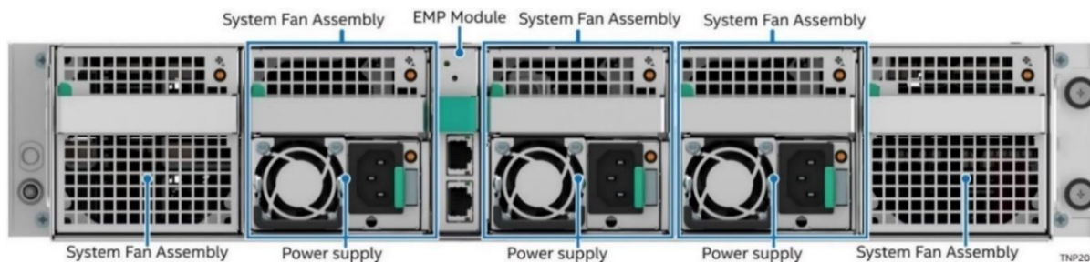
Figure 45. Air-Cooled System Back View
