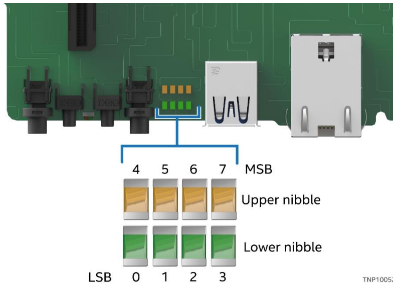
Figure 6. Onboard LED Location
