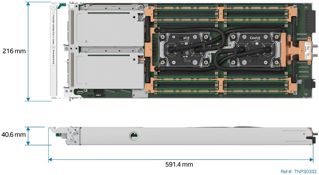
Figure 108. 1U Liquid-Cooled Compute Module Dimensions
