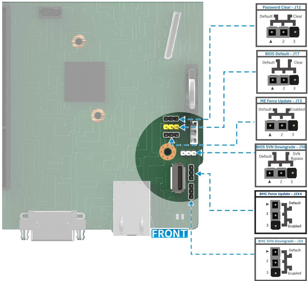
Figure 5. Reset and Recovery Jumper Header Location
