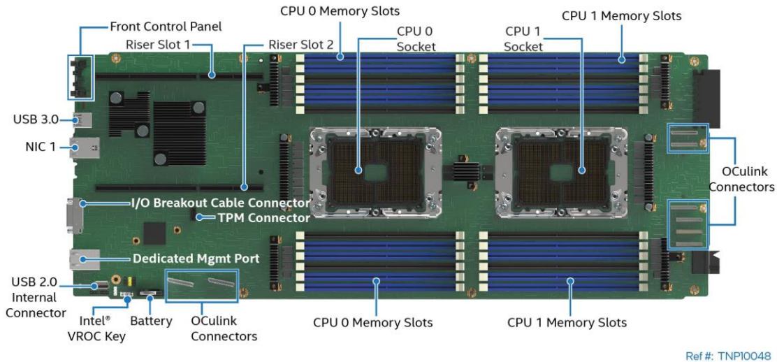
Figure 3. Intel® Server Board D50TNP1SB Feature Identification
