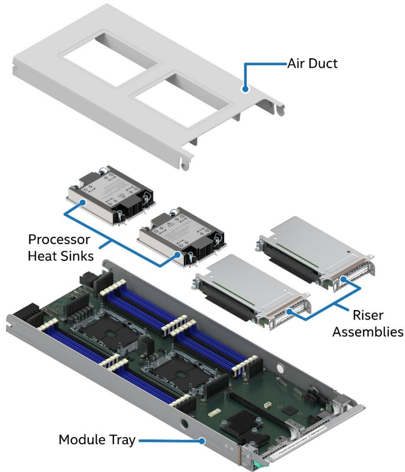
Figure 16. 1U Air-Cooled Compute Module Components (Standard Heat Sinks Shown)
