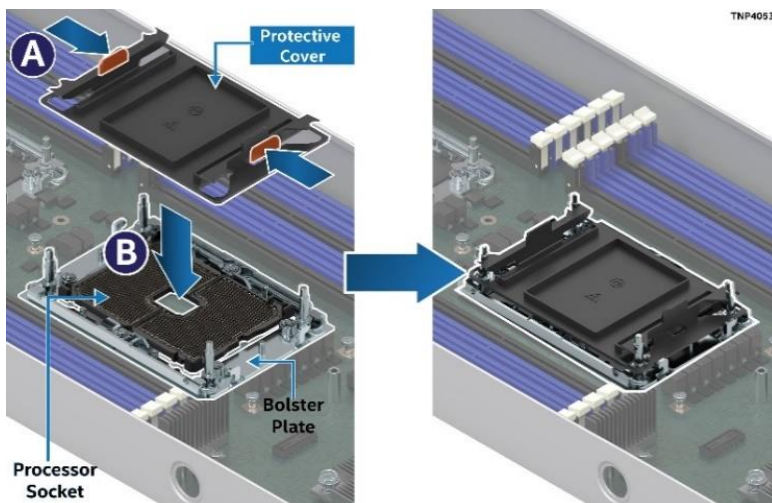
Figure 130. Reinstall the Socket Cover
