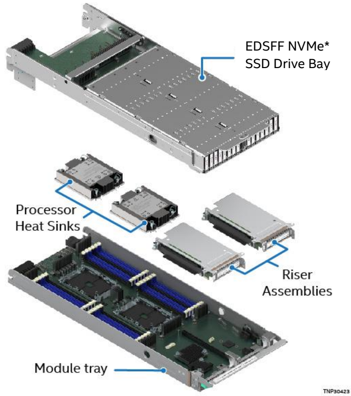
Figure 30. 2U Storage Module Components
