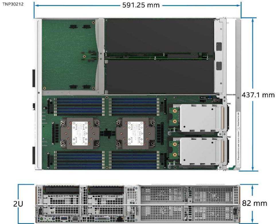
Figure 112. 2U Accelerator Module Dimensions
