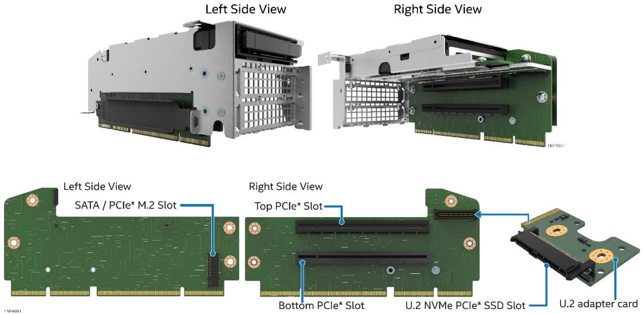
Figure 20. 2U Riser Card Assembly
