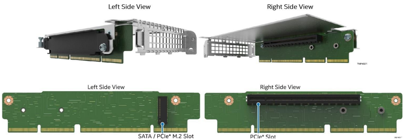
Figure 12. 1U Riser Card Assembly (D50TNP1MHCPAC)
