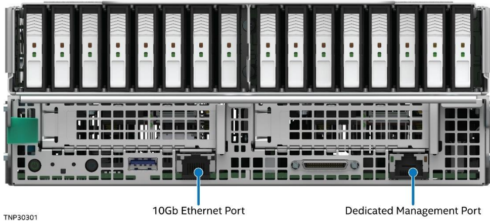
Figure 72. RJ45 Connector Identification – 2U Storage Module
