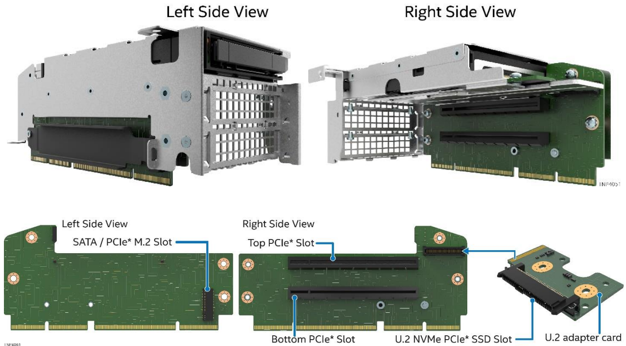
Figure 35. 2U Riser Card Assembly
