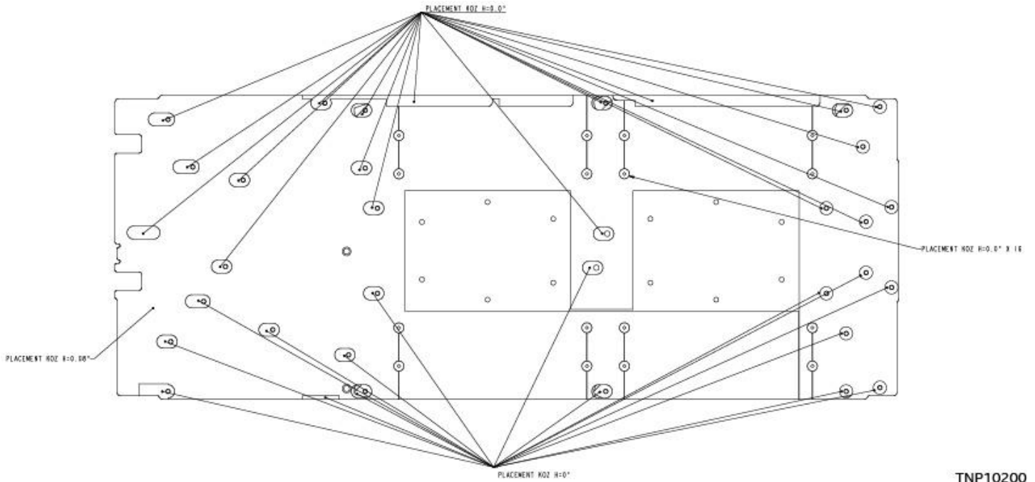
Figure 122. Intel® Server Board D50TNP1SBCR Bottom Surface Keep Out zone
