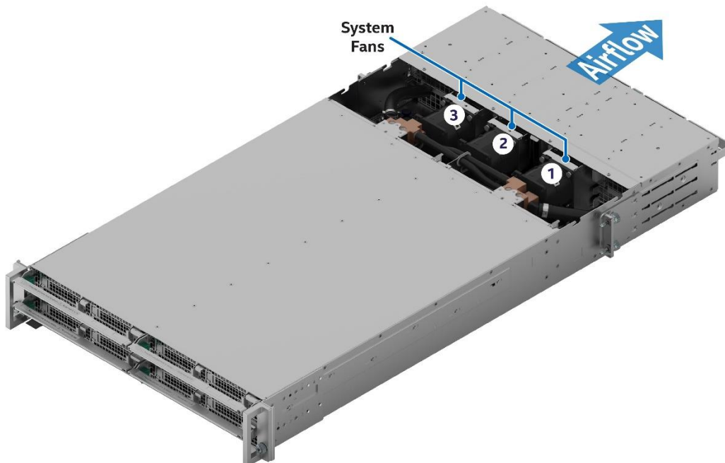
Figure 82. Liquid-Cooled System Airflow and Fan Identification
