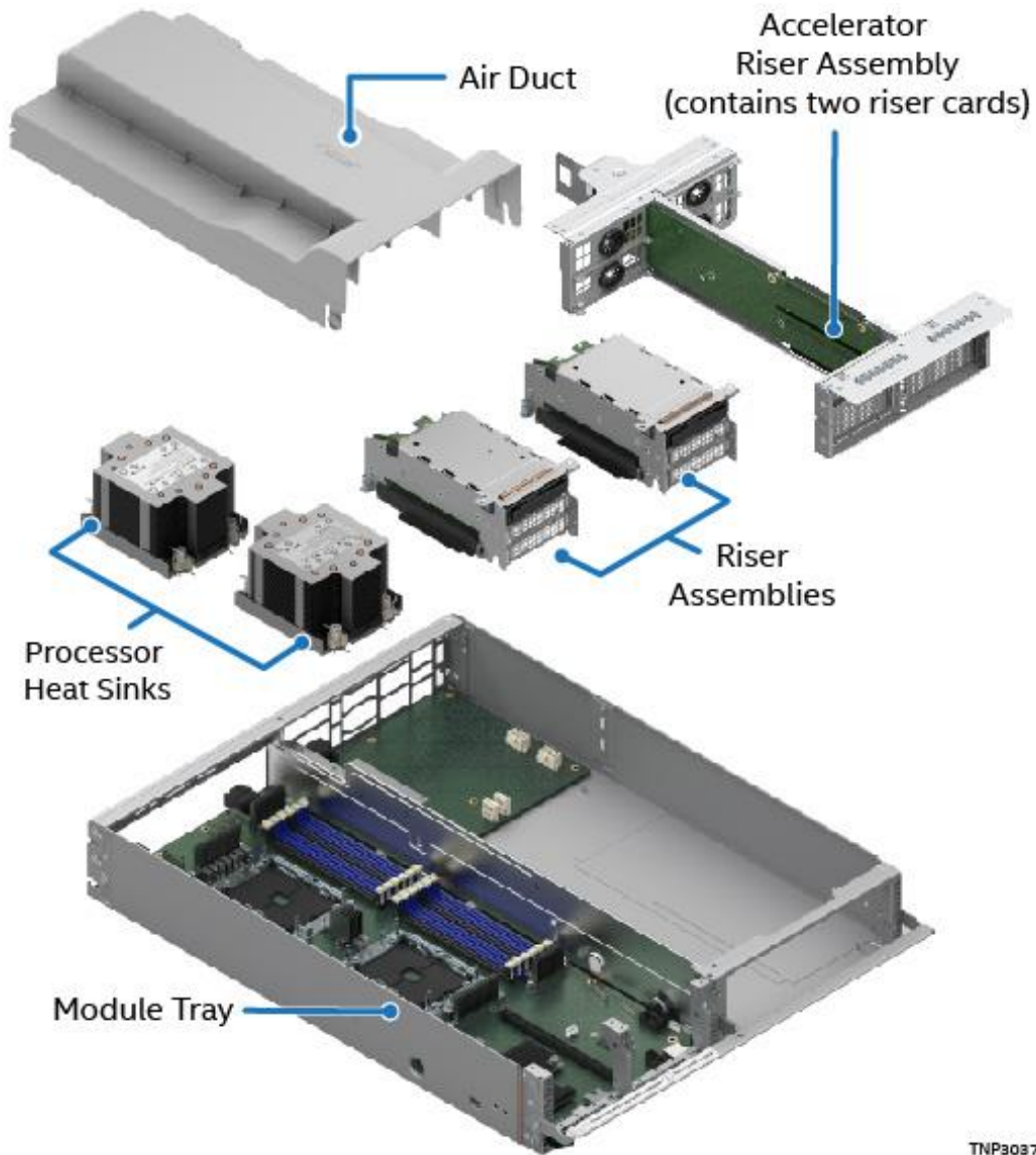
Figure 37. 2U Accelerator Module Components
