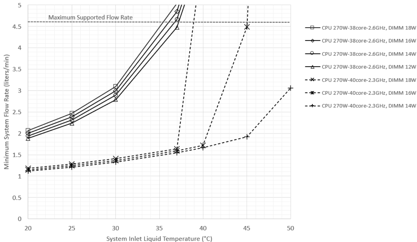
Figure 87. System Coolant Flow Rate Requirements
