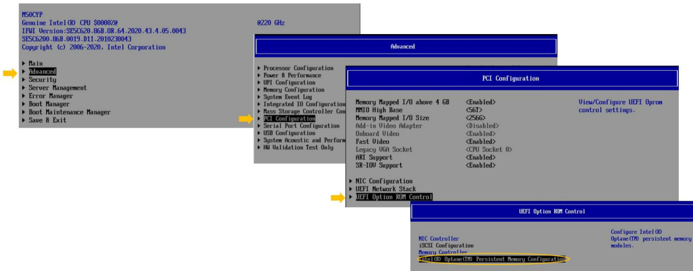
Figure 56. <F2> BIOS Setup Screen Navigation for Intel® Optane™ PMem Setup Options
