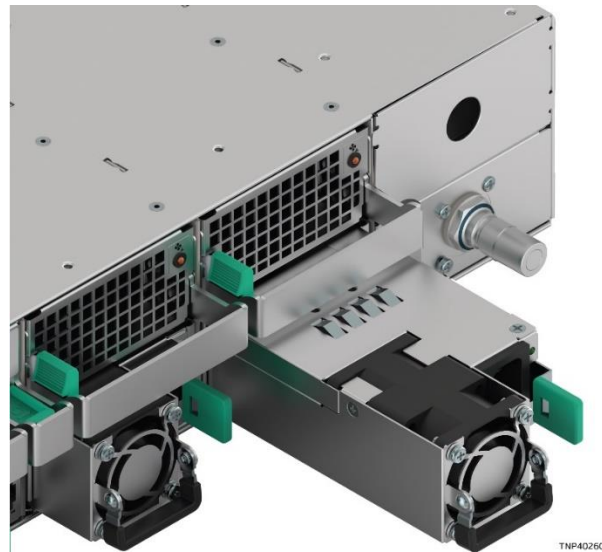
Figure 90. Power Supply Module Partially Out of Chassis
