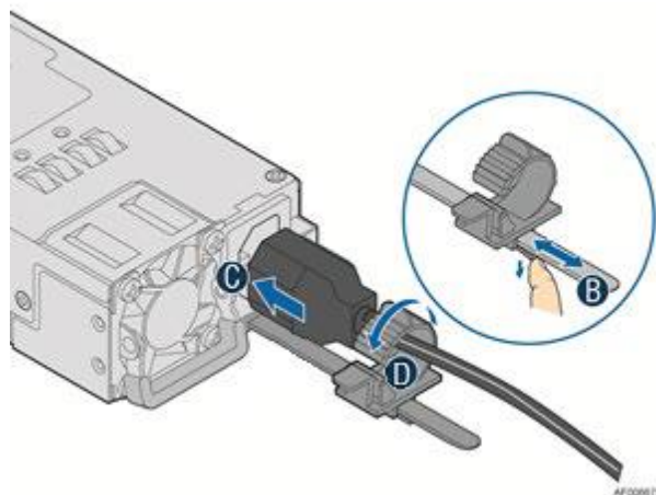
Figure 92. Power Cord Retention Strap
