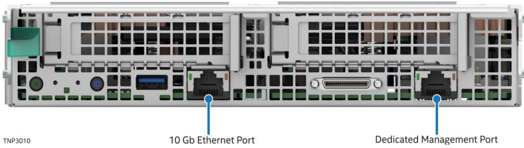
Figure 70. RJ45 Connector Identification – 1U Compute Module
