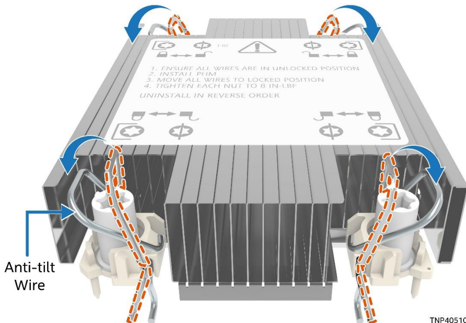
Figure 136. Processor Heat Sink Anti-tilt Wires in the Outward Position
