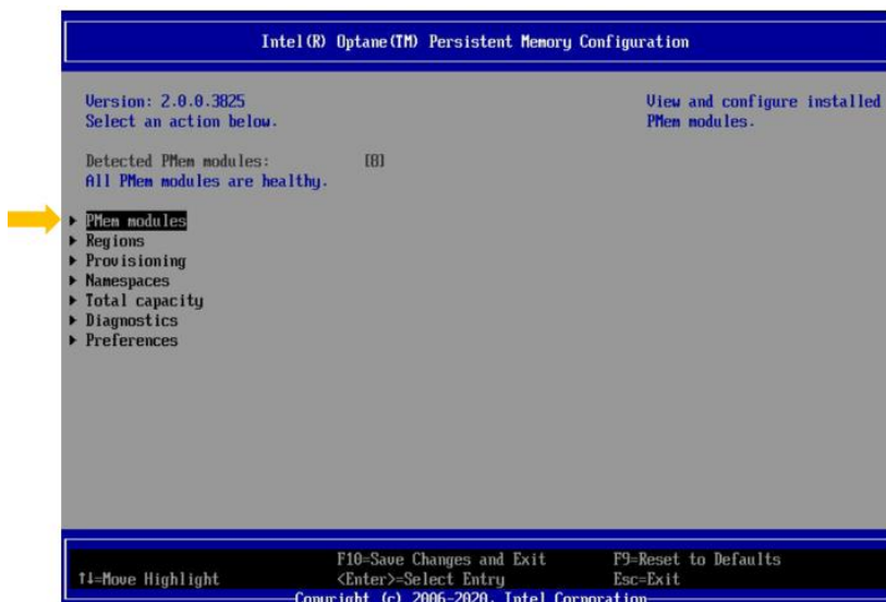
Figure 57. Intel® Optane™ PMem Configuration Menu in <F2> BIOS Setup
