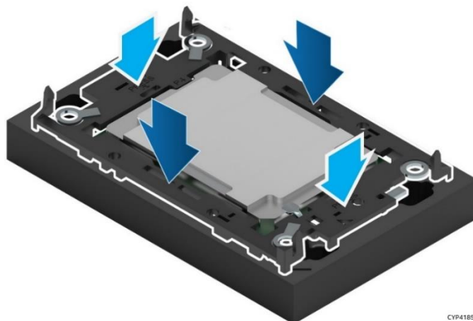
Figure 134. Installing Processor Carrier Clip onto Processor – Part 2
