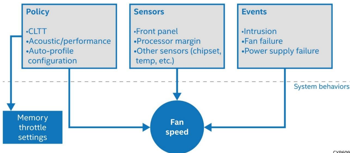
Figure 84. High-Level Fan Speed Control Model
