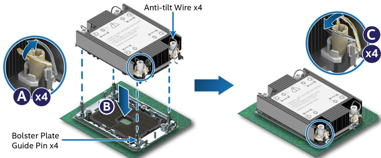
Figure 140. PHM Installation onto Server Board
