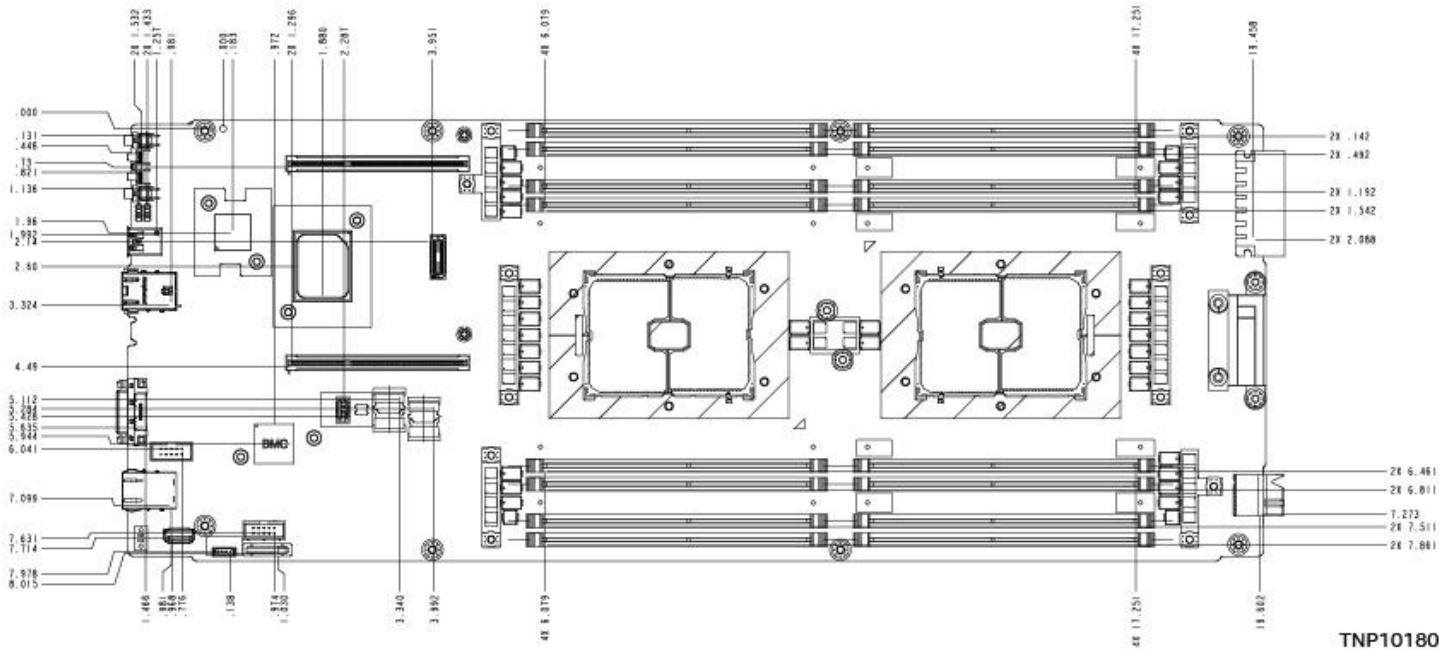
Figure 124. Intel® Server Board D50TNP1SBCR Holes Position
