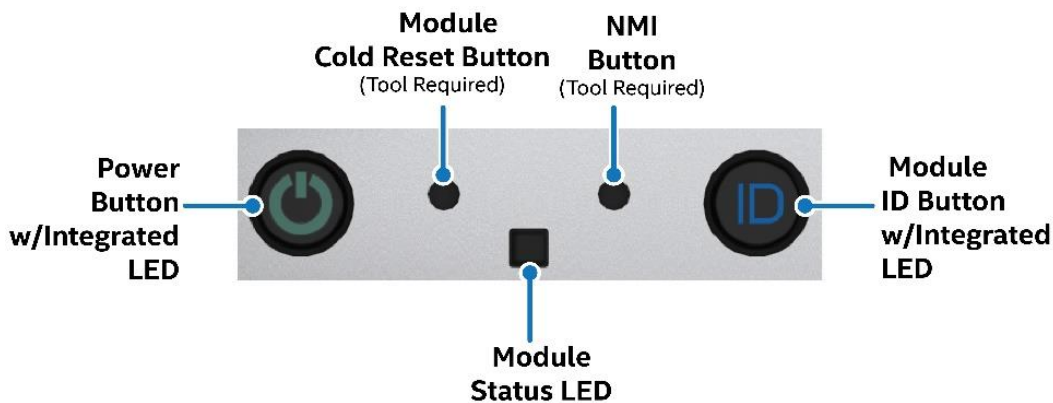
Figure 7. Front Control Panel Features
