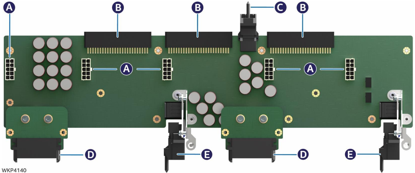
Figure 96. Power Distribution Board Connector Identification
