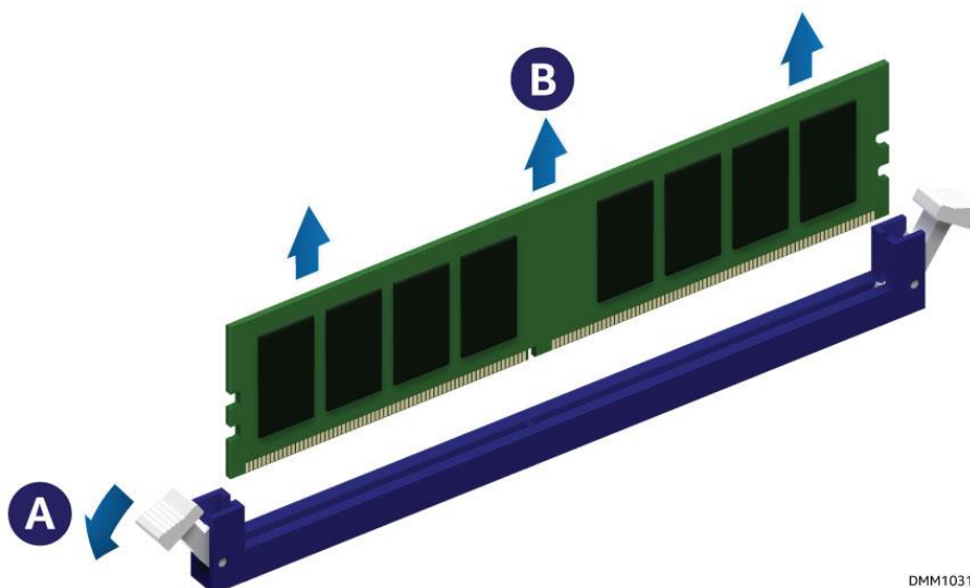
Figure 142. Removing the DIMM from an Air-Cooled System
