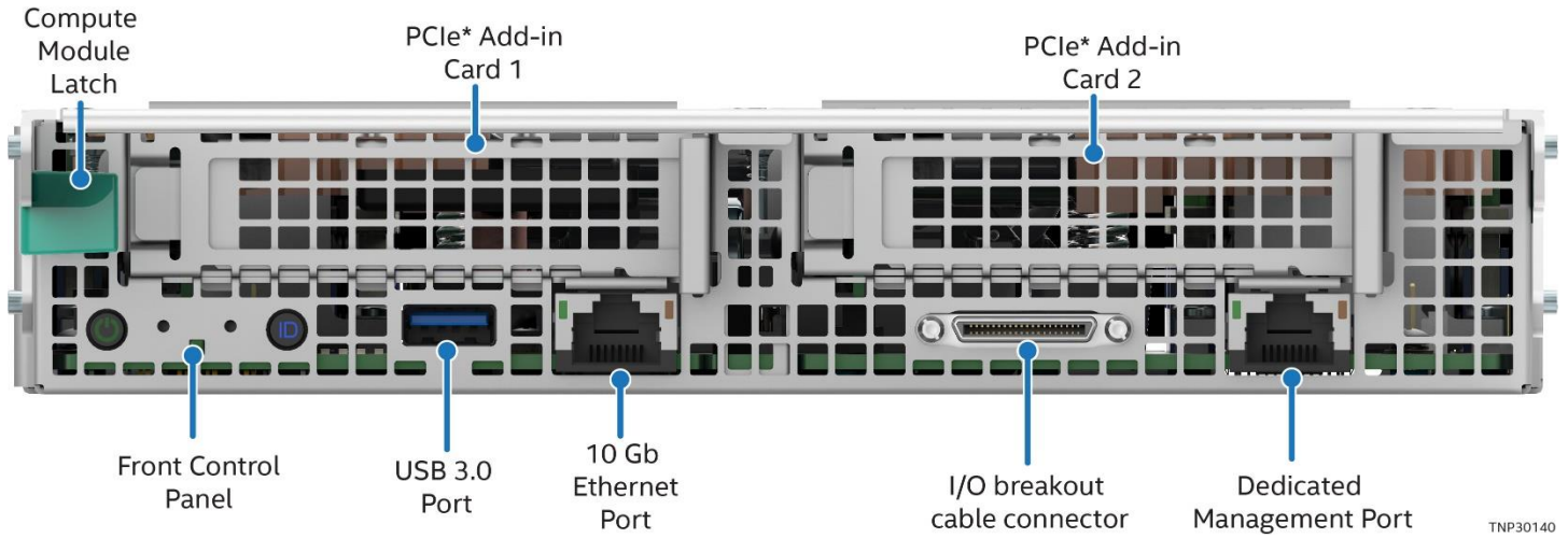
Figure 14. 1U Compute Module Front Panel Features
