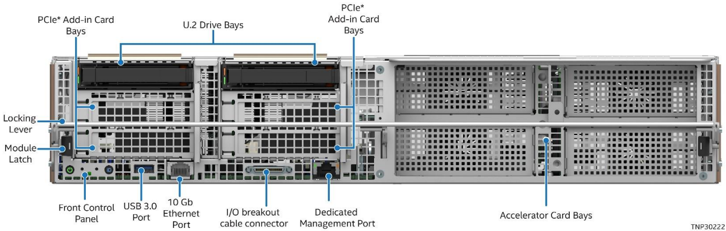
Figure 36. 2U Accelerator Module Front Panel Features
