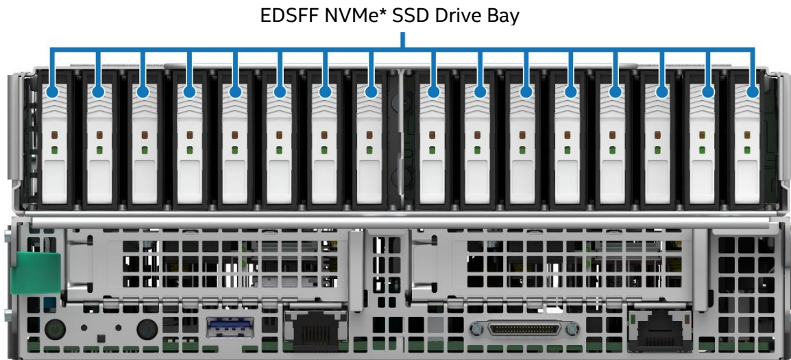
Figure 25. EDSFF NVMe* Drive Bay – 2U Storage Modules
