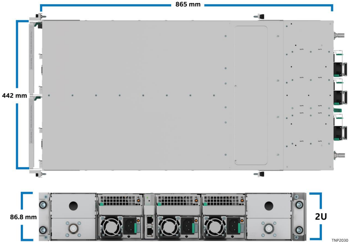
Figure 113. System chassis Dimensions
