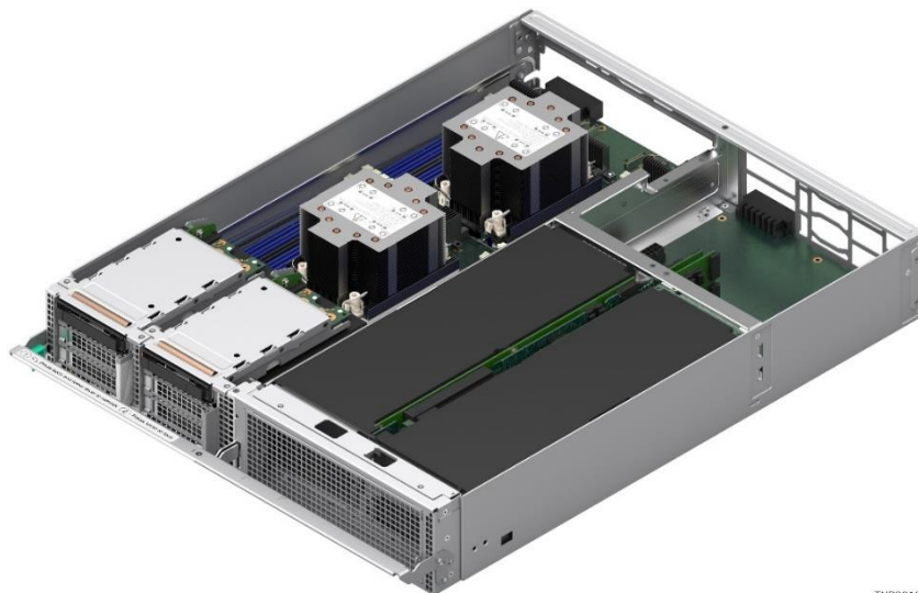
Figure 32. Air-Cooled Accelerator Module
