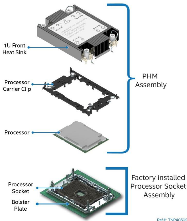
Figure 46. PHM Components and Processor Socket Reference Diagram
