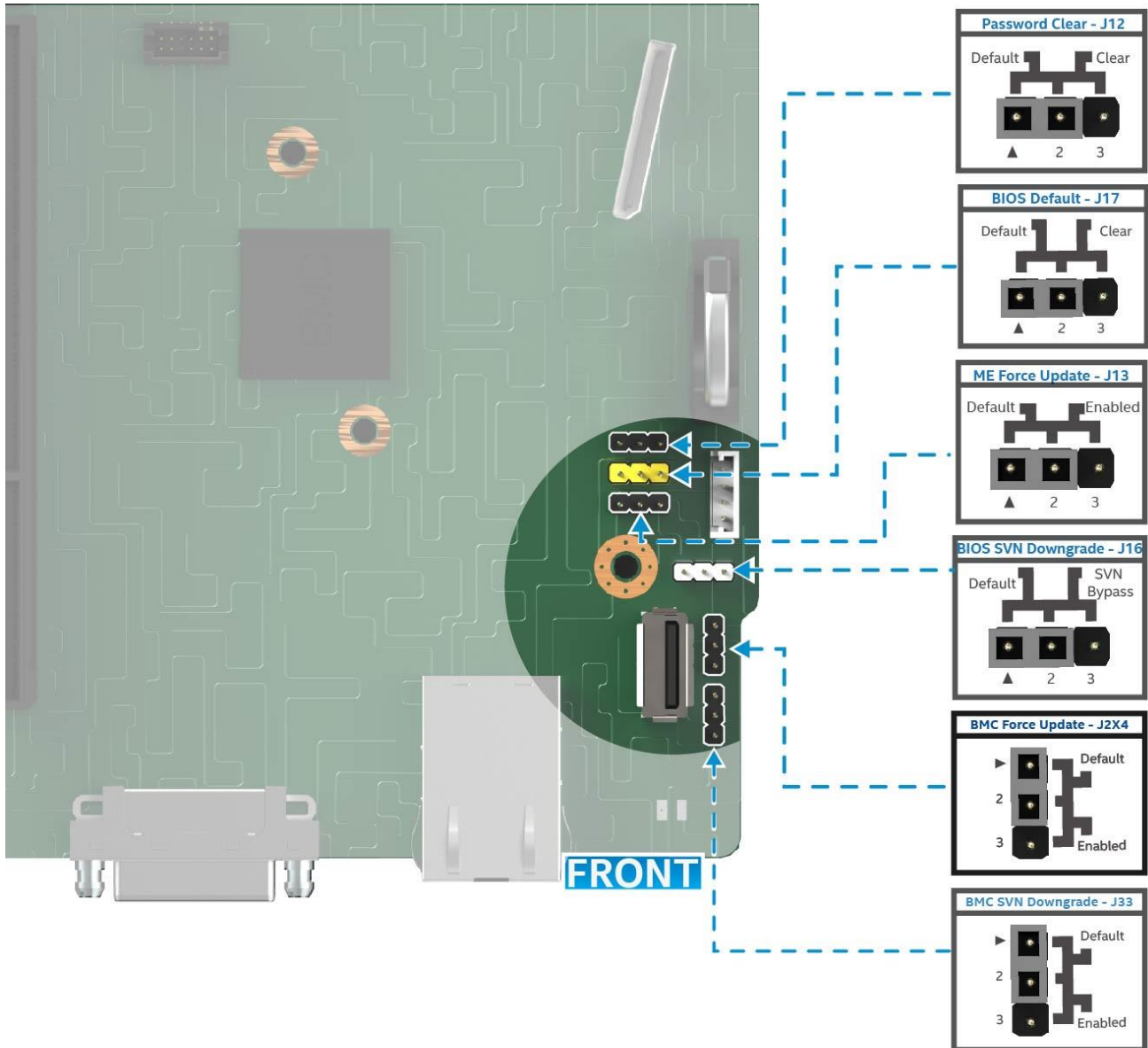
Figure 106. Reset and Recovery Jumper Block Location
