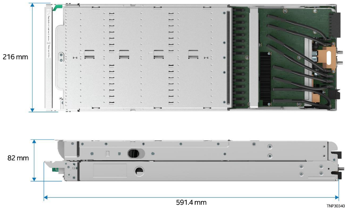
Figure 111. 2U Storage Module Dimensions
