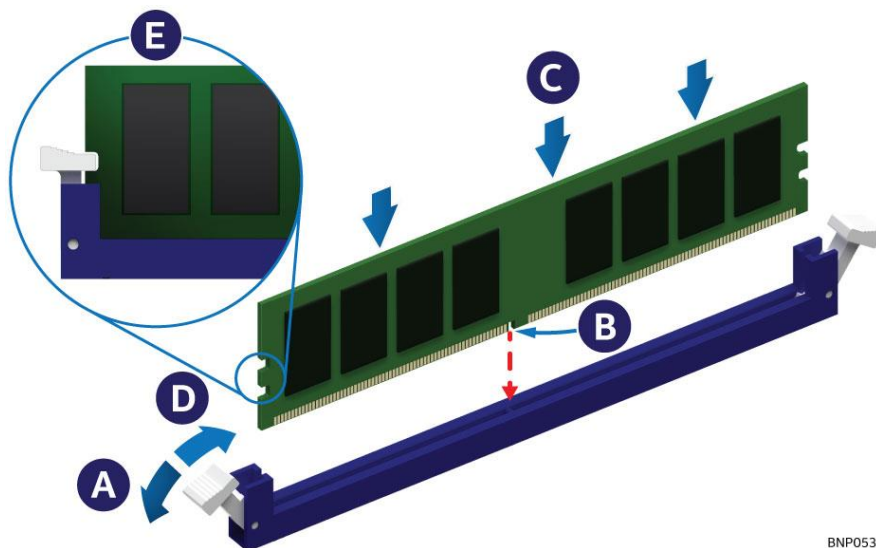
Figure 143. Installing the DIMM in an Air-Cooled System
