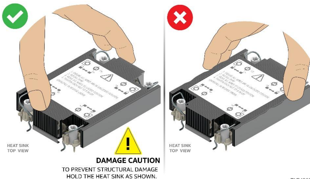
Figure 135. Processor Heat Sink Handling
