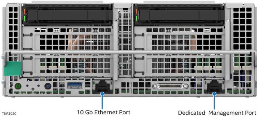
Figure 71. RJ45 Connector Identification – 2U Management Module
