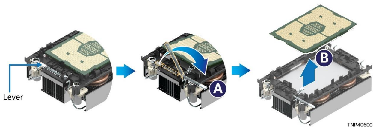
Figure 131. Processor Removal from PHM Assembly
