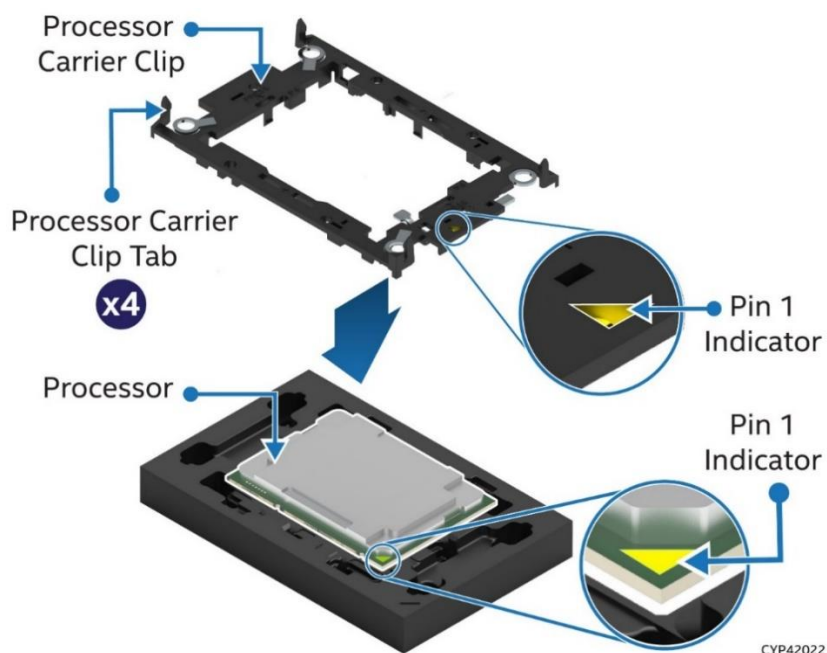
Figure 133. Installing Processor Carrier Clip onto Processor – Part 1
