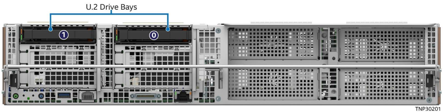
Figure 64. U.2 Drive Bay Identification – 2U Accelerator Module
