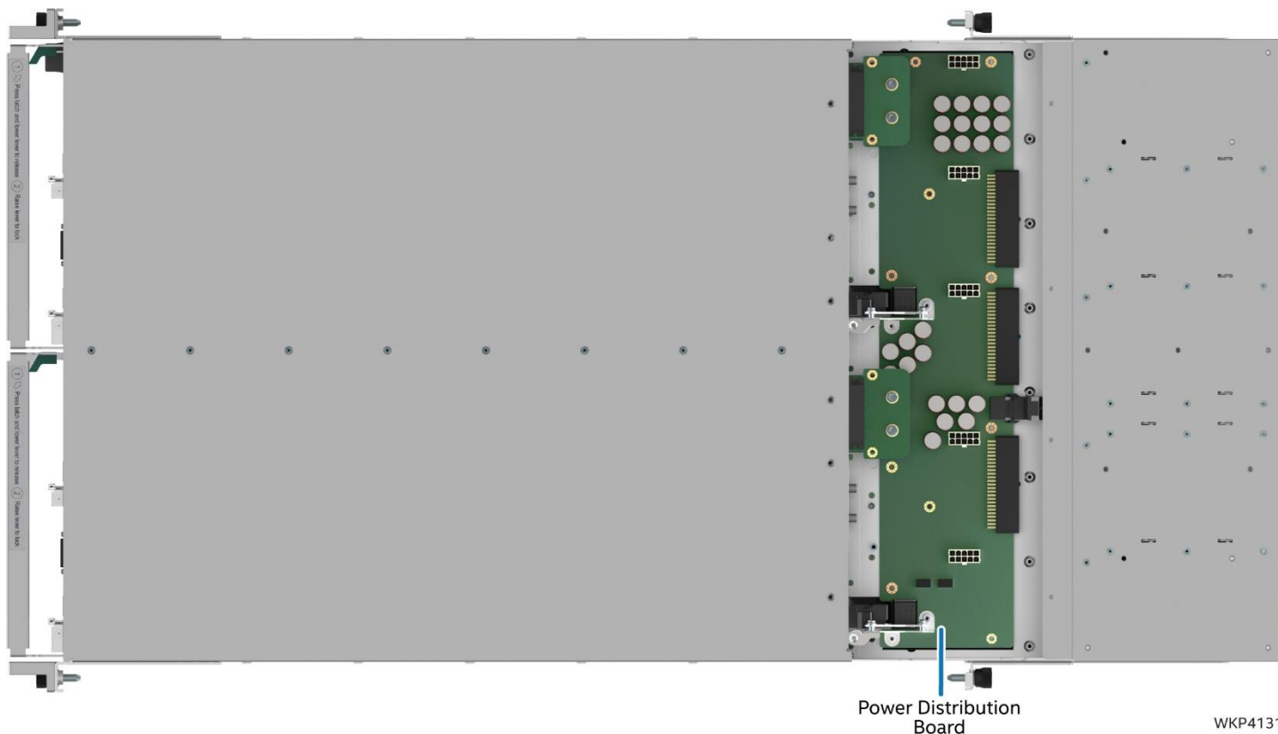
Figure 95. Power Distribution Board Identification
