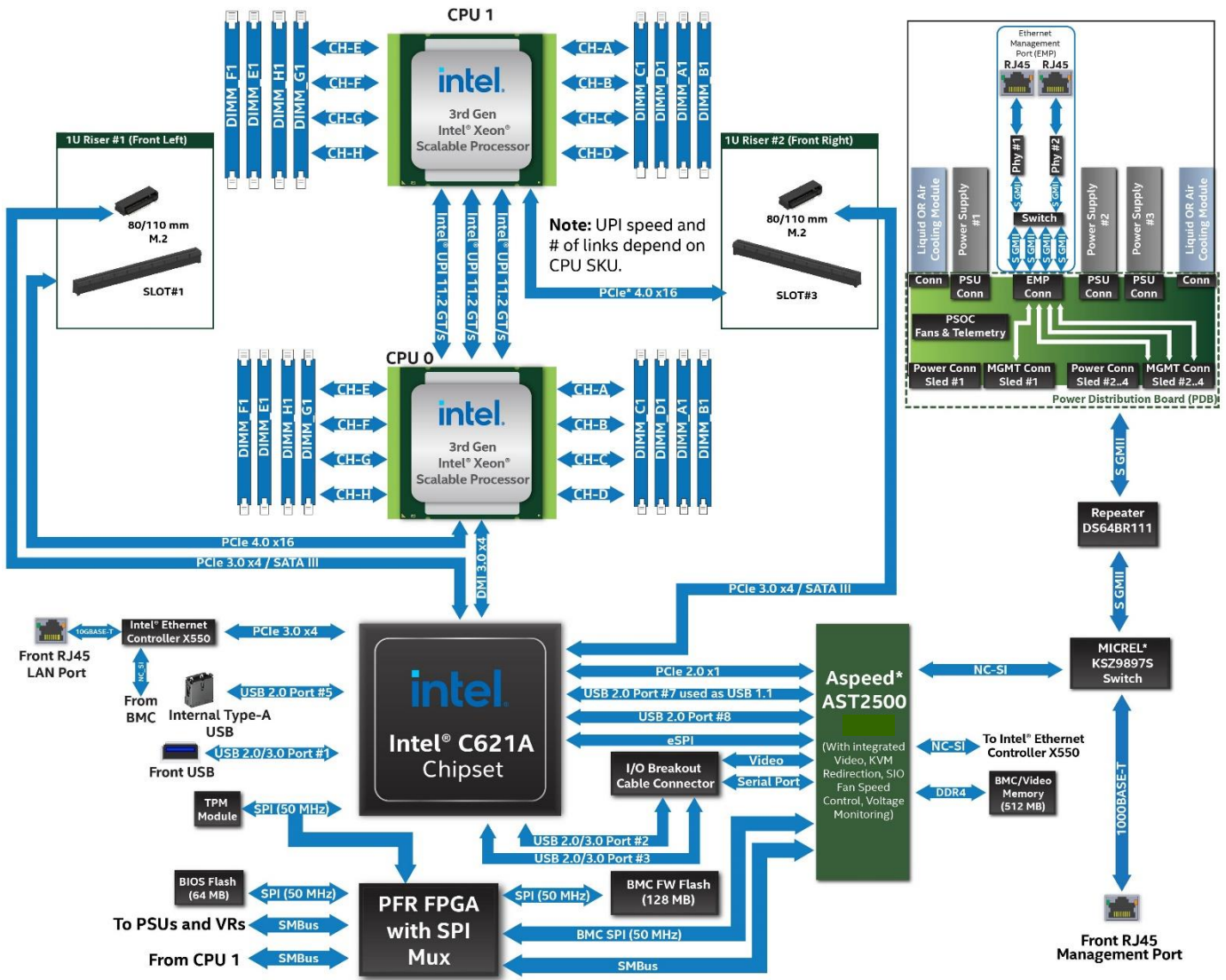
Figure 9. Intel® Server Board D50TNP1SBCR Architectural Block Diagram
