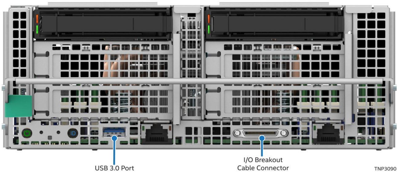
Figure 78. USB Port Location - 2U Management Module
