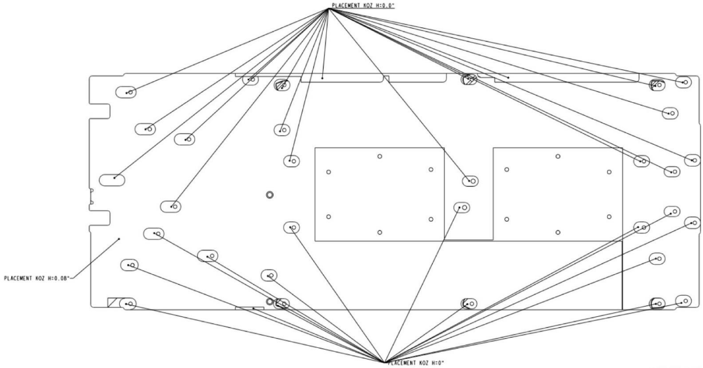
Figure 118. Intel® Server Board D50TNP1SB Bottom Surface Keep Out Zone
