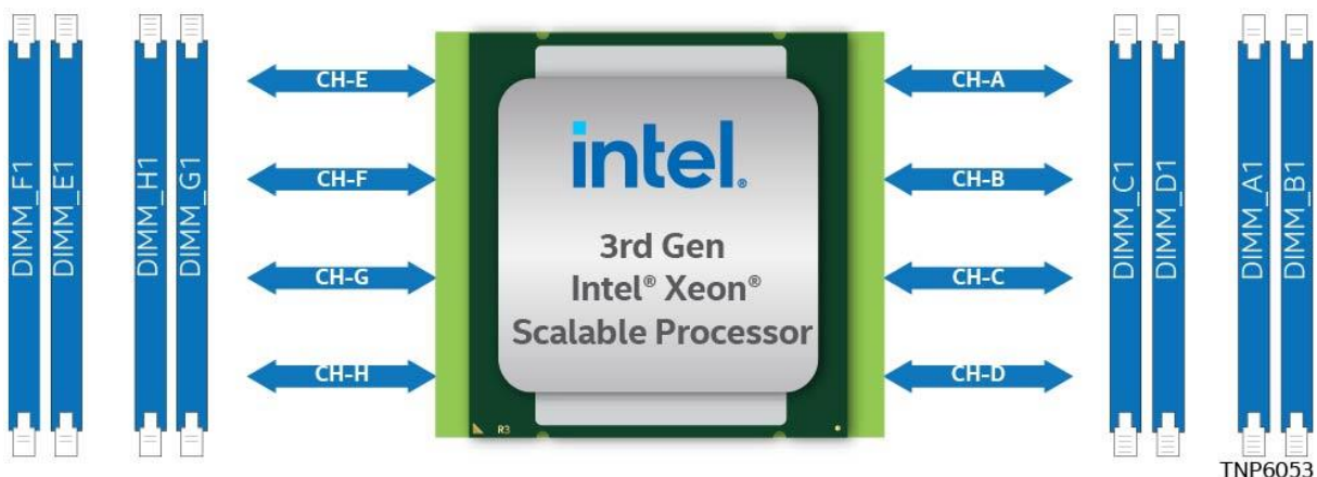
Figure 53. Memory Slot Connectivity for D50TNP1SBCR
