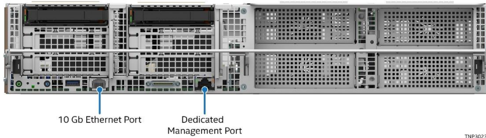
Figure 73. RJ45 Connector Identification – 2U Accelerator Module
