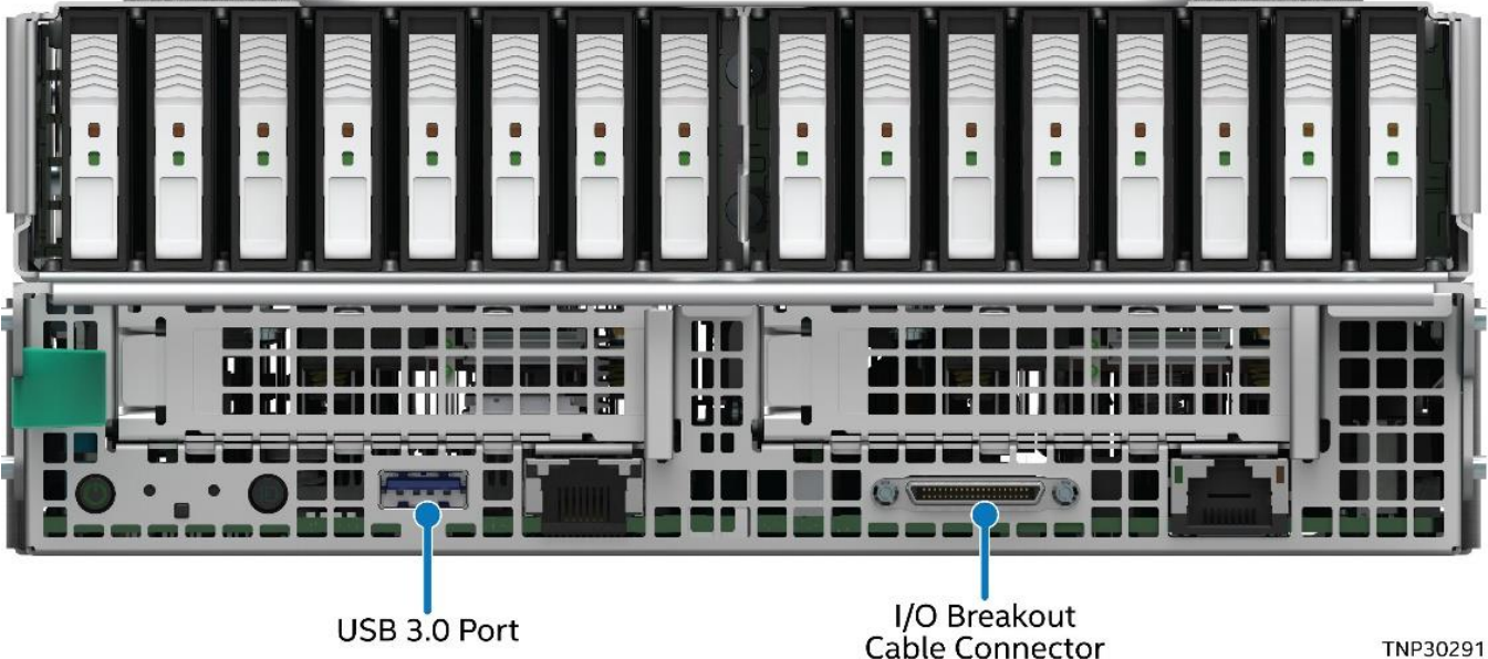
Figure 79. USB Port Location - 2U Storage Module
