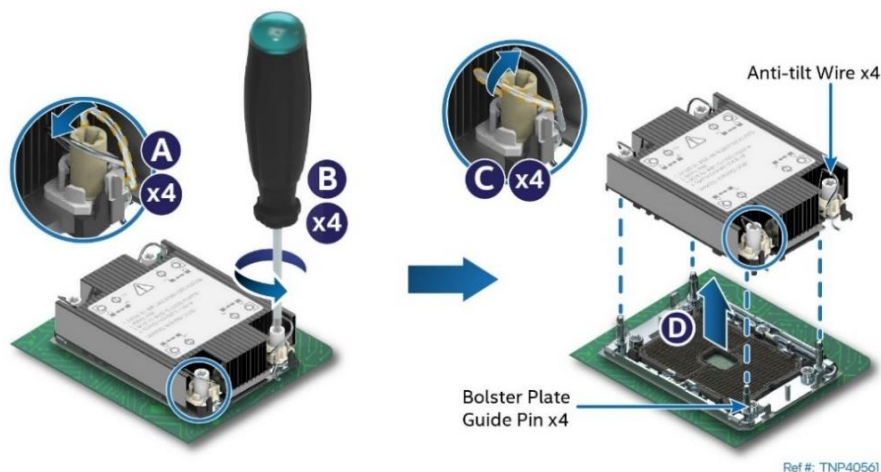
Figure 129. PHM Assembly Removal from Processor Socket
