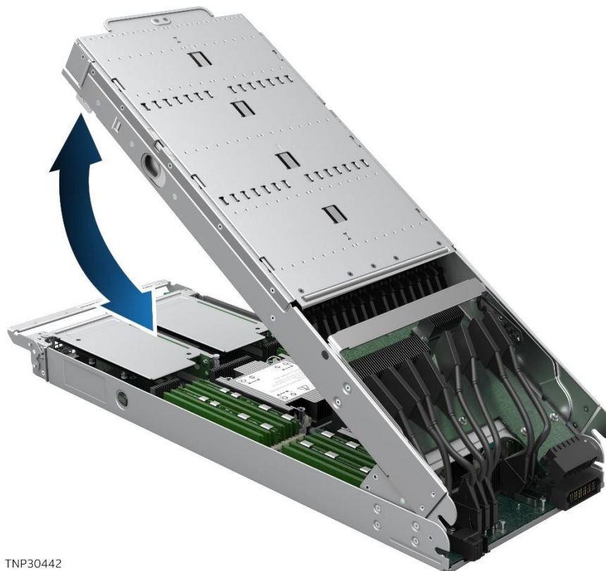
Figure 26. Air-Cooled Storage Module -- Service View
