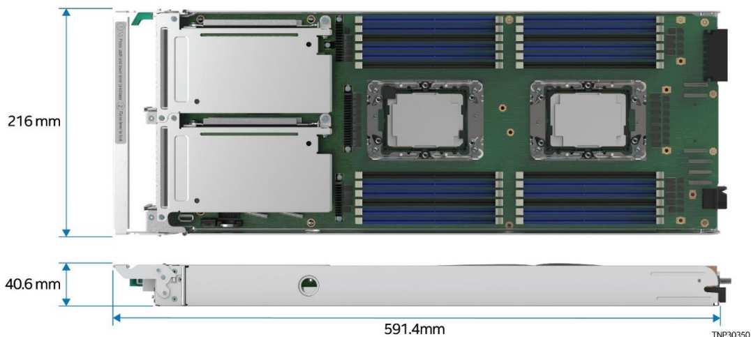
Figure 18. 1U Air-Cooled Compute Module Dimensions
