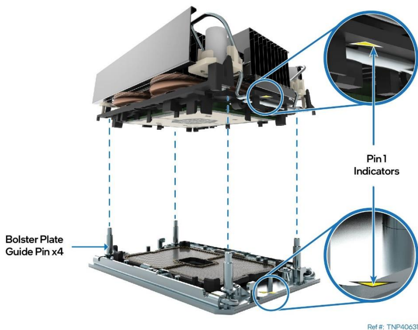
Figure 139. PHM Alignment with Socket Assembly
