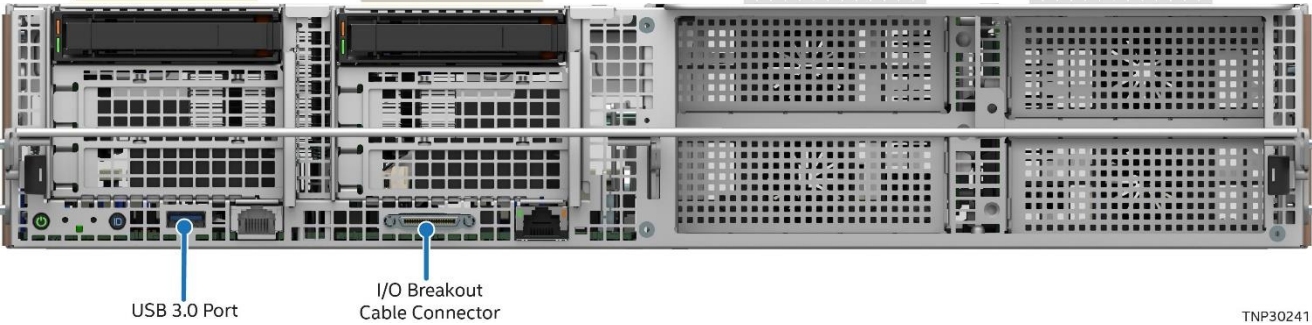
Figure 80. USB Port Location - 2U Accelerator Module
