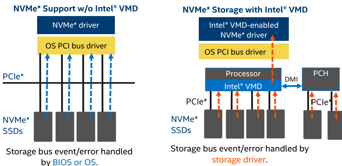
Figure 67. NVMe* Storage Bus Event / Error Handling
