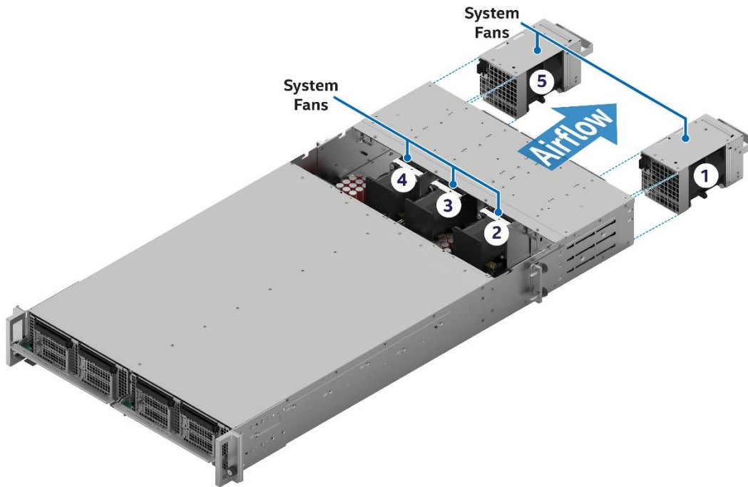
Figure 81. Air-Cooled System Airflow and Fan Identification
