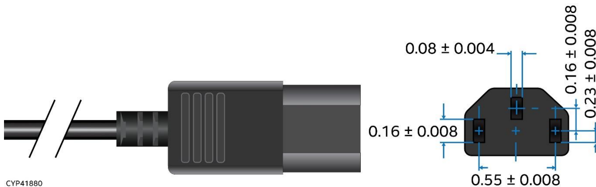
Figure 94. AC Power Cord Specification
