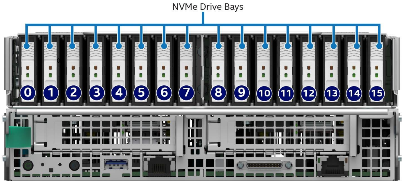
Figure 66. EDSFF NVMe* SSD Drive Identification – 2U Storage Modules
