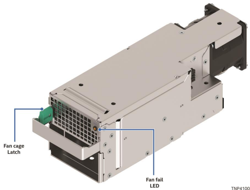
Figure 83. System Fan Cage Assembly
