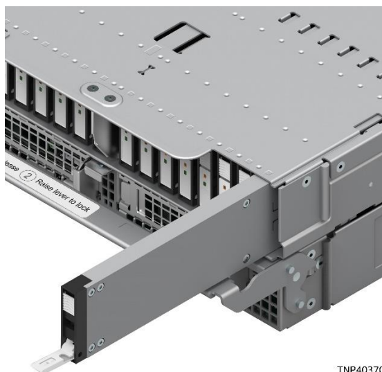
Figure 27. EDSFF NVMe* SSD in Air-Cooled Storage Module
