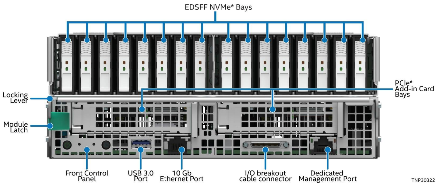
Figure 29. 2U Storage Module Front Panel Features
