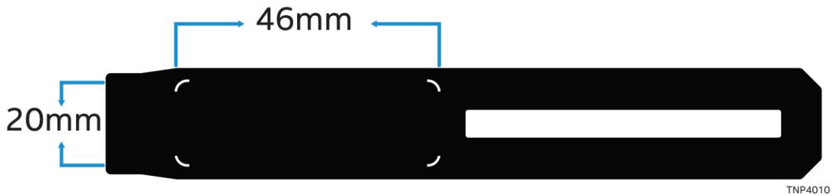
Figure 115. Pull-out Tab Dimensions
