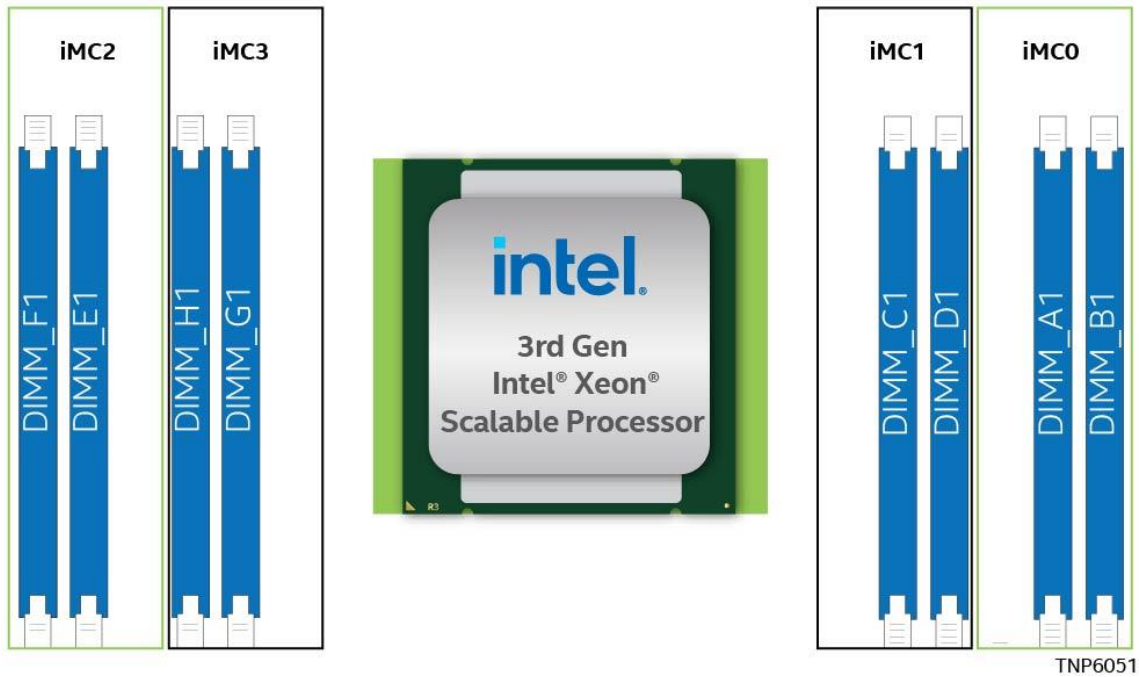
Figure 61. Memory Slot Identification for Intel® D50TNP Modules with D50TNP1SBCR Server Board
