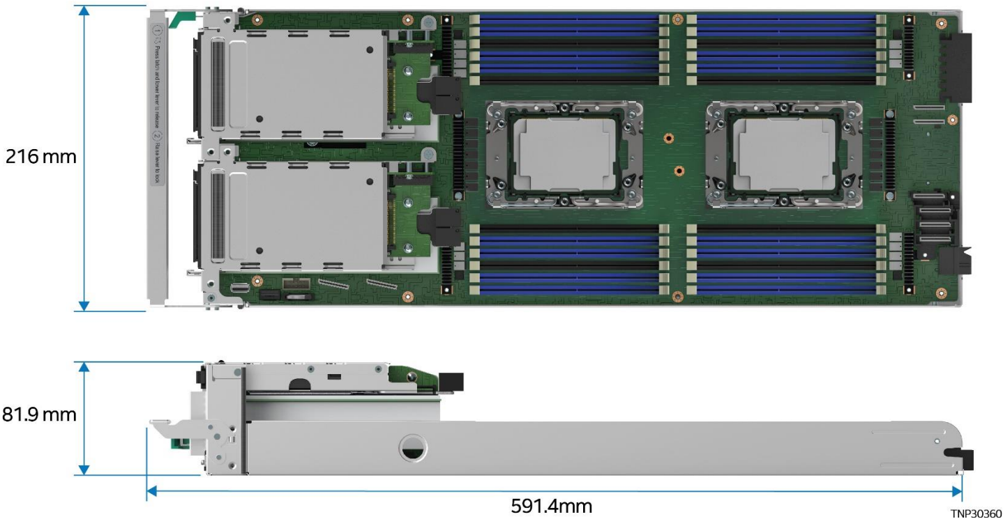
Figure 110. 2U Management Module Dimensions
