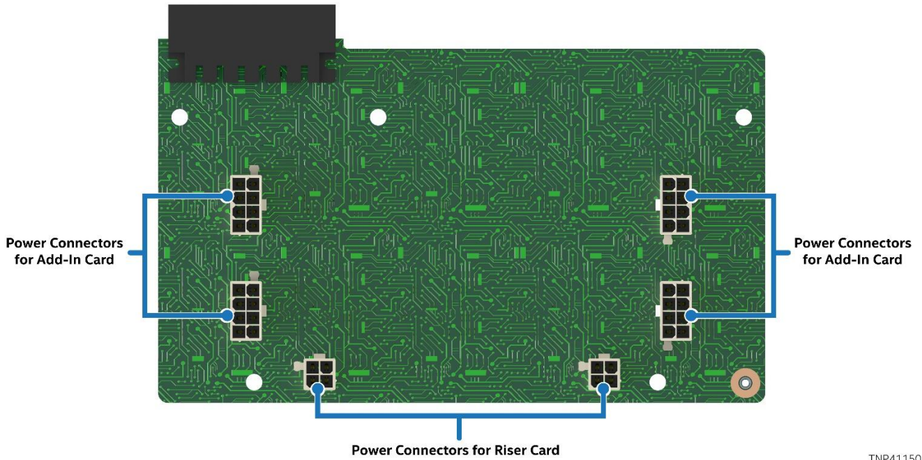
Figure 34. Power Connector Board for Accelerator Module
