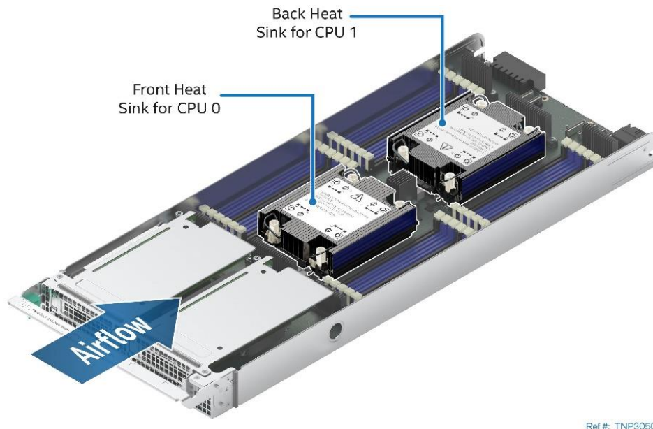
Figure 50. 1U Heat Sinks Installed in Module
