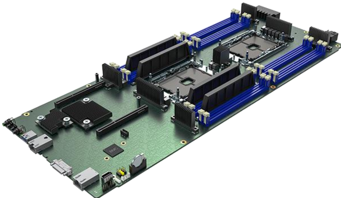
Figure 2. Intel® Server Board D50TNP1SBCR
