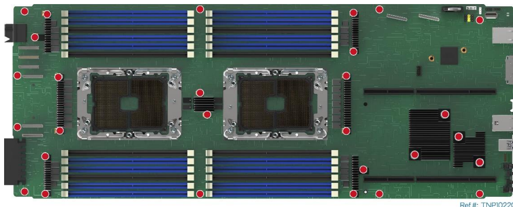
Figure 126. Server Board Mounting Hole Locations
