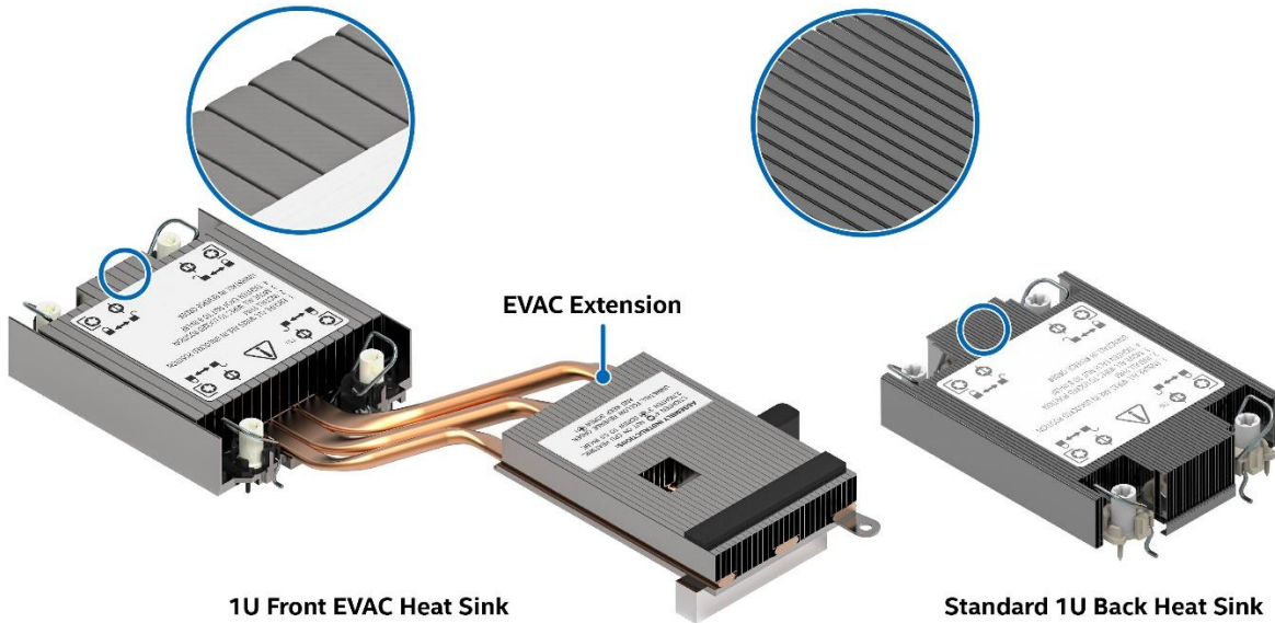
Figure 48. 1U Supported EVAC Processor Heat Sinks
