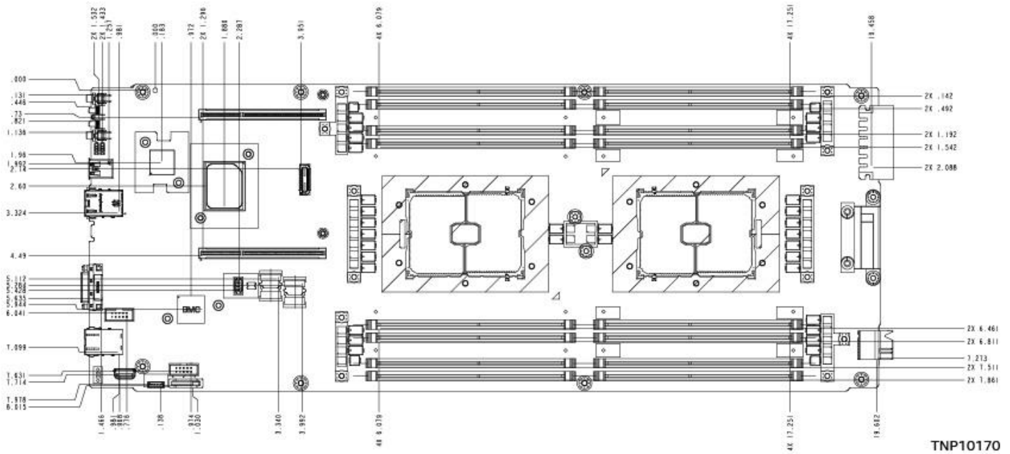
Figure 123. Intel® Server Board D50TNP1SBCR Components Position
