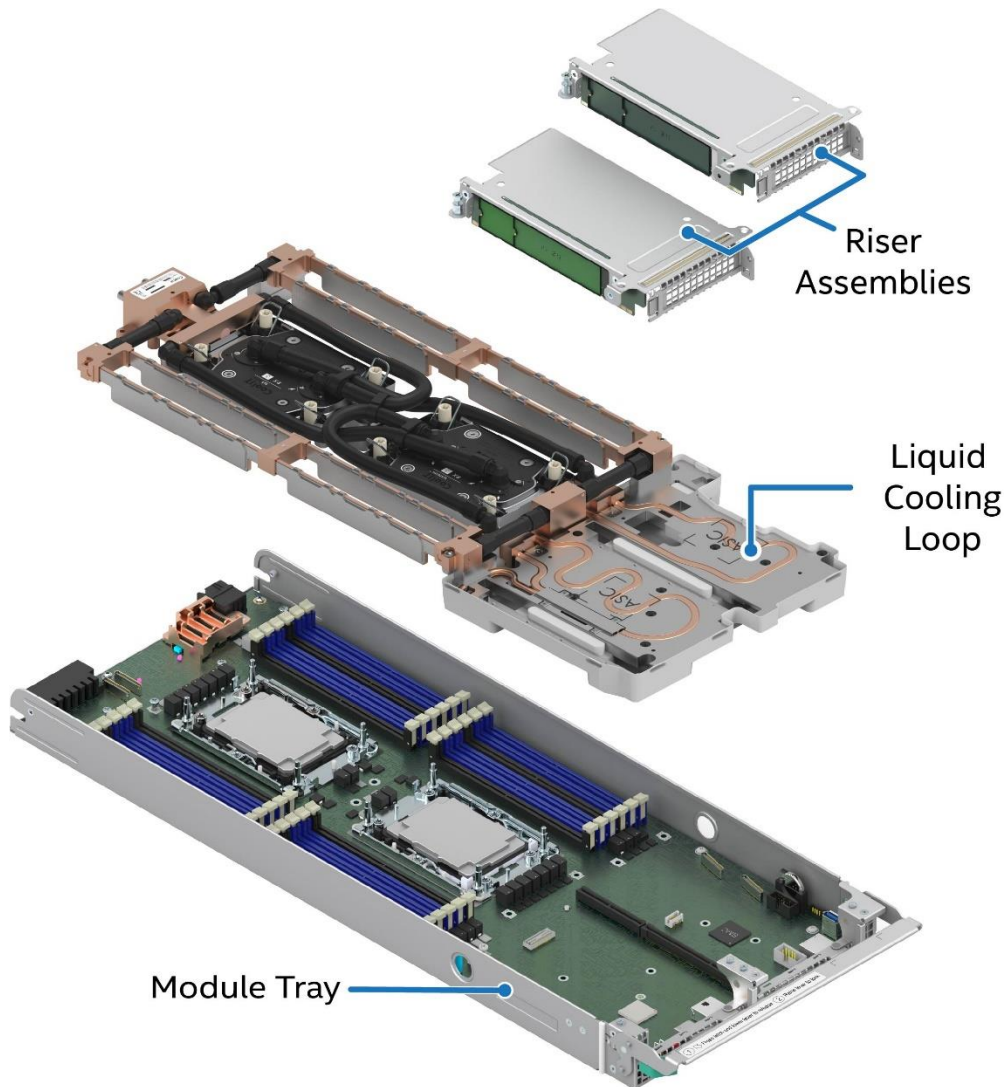
Figure 15. 1U Liquid-Cooled Compute Module Components
