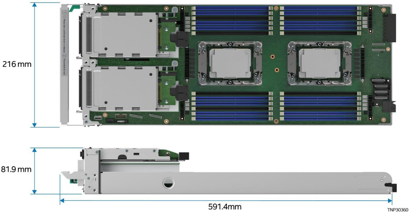
Figure 23. 2U Management Module Dimensions
