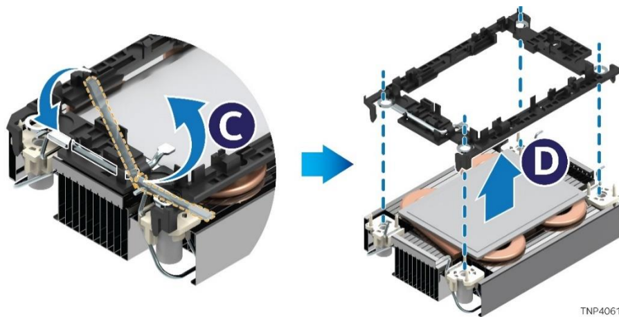
Figure 132. Processor Carrier Clip Removal from PHM Assembly
