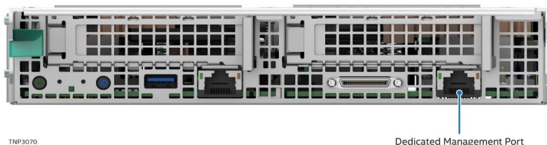
Figure 97. Dedicated Management Port Location – 1U Compute Modules
