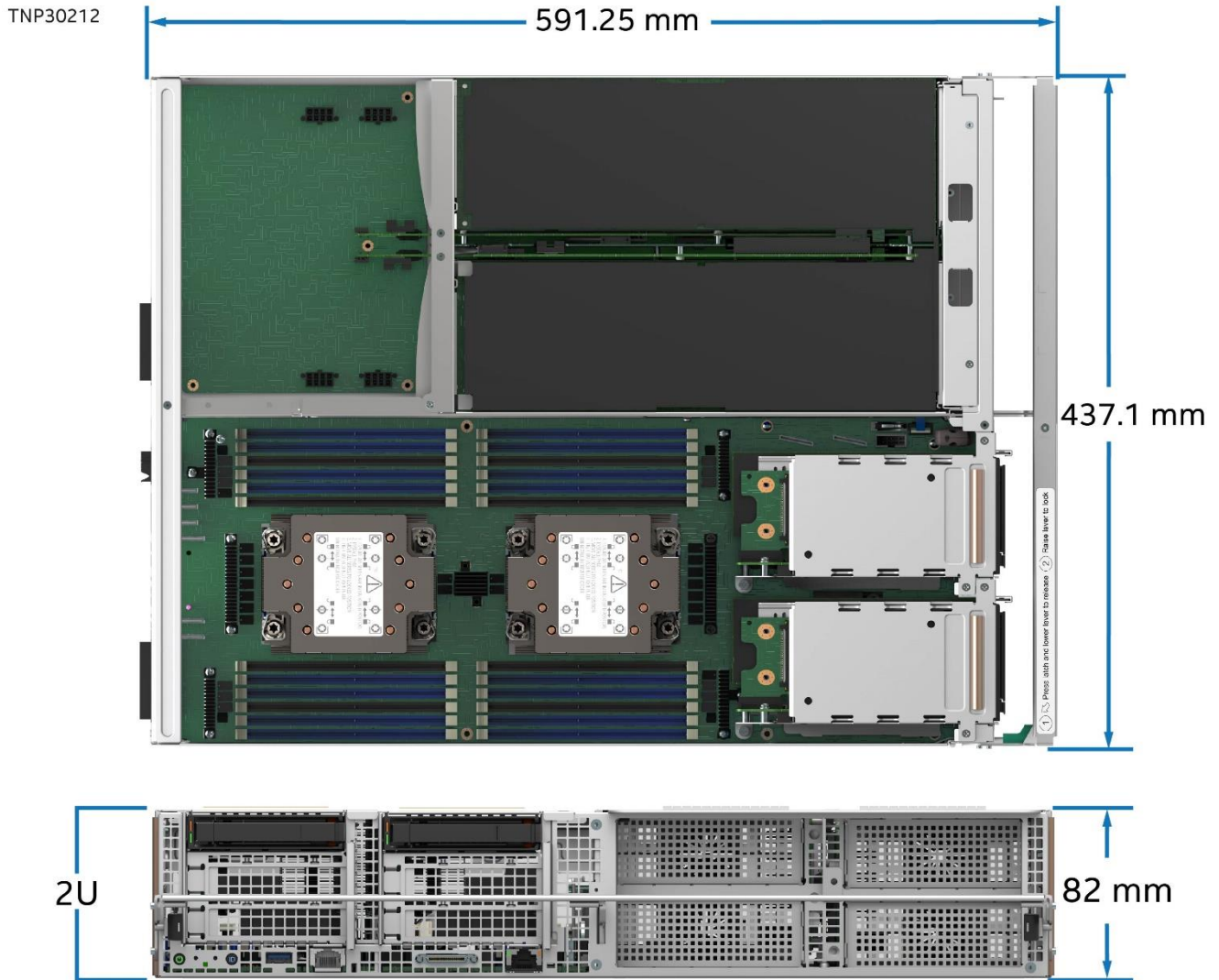
Figure 38. 2U Accelerator Module Dimensions
