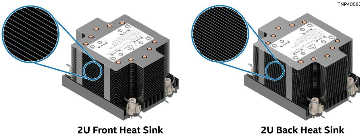
Figure 49. 2U Supported Processor Heat Sinks
