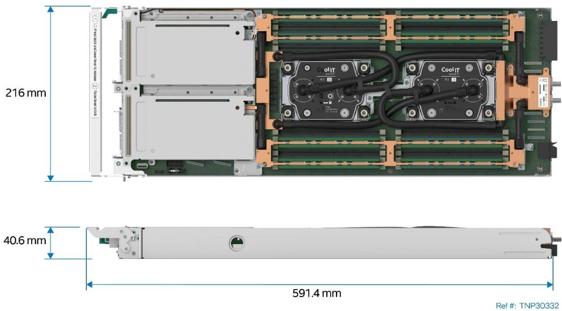
Figure 17. 1U Liquid-Cooled Compute Module Dimensions
