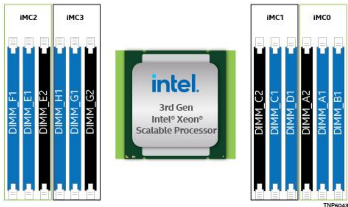
Figure 60. Memory Slot Identification for Intel® D50TNP Modules with D50TNP1SB Server Board
