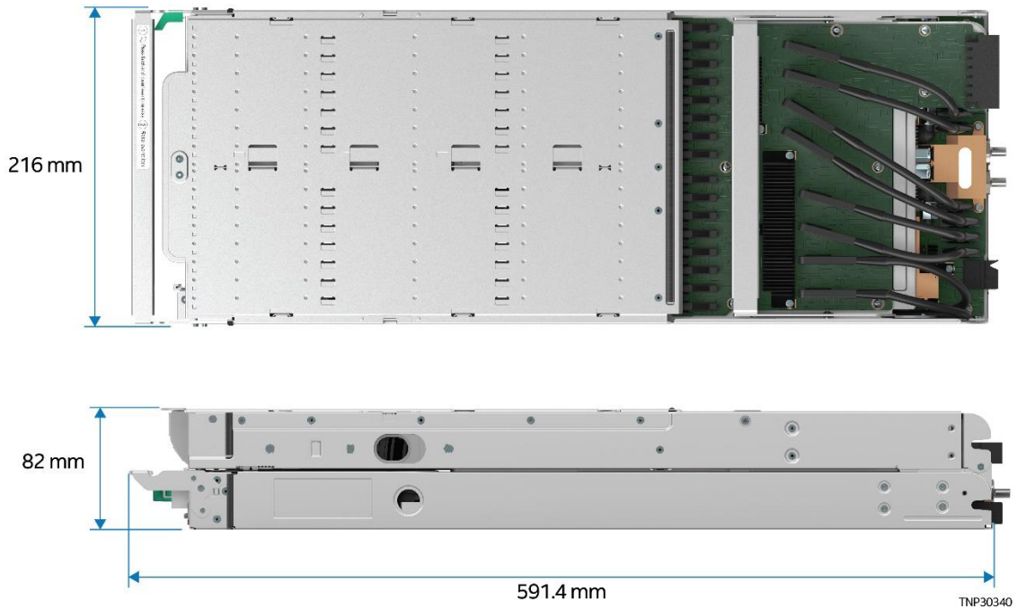
Figure 31. 2U Storage Module Dimensions
