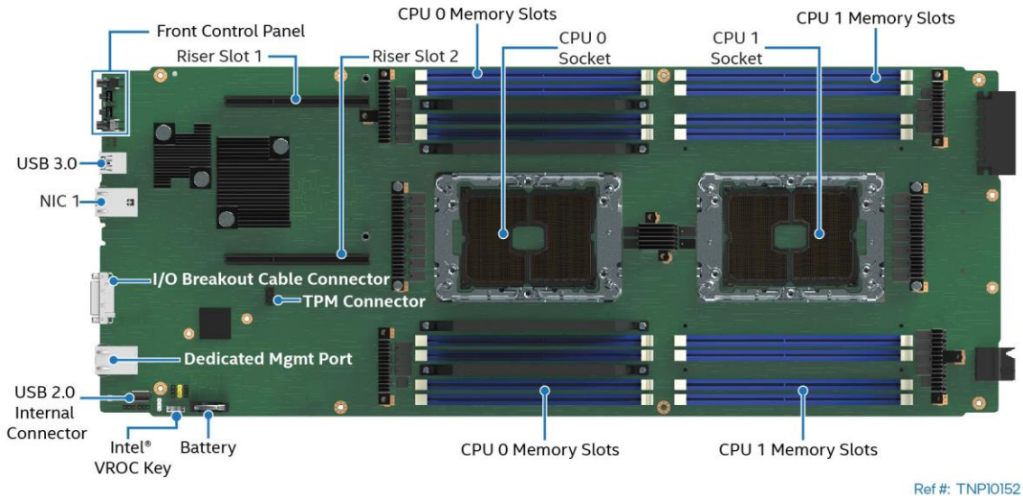
Figure 4. Intel® Server Board D50TNP1SBCR Feature Identification
