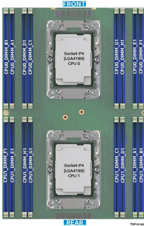
Figure 59. Intel® Server Board D50TNP1SBCR Memory Slot Layout
