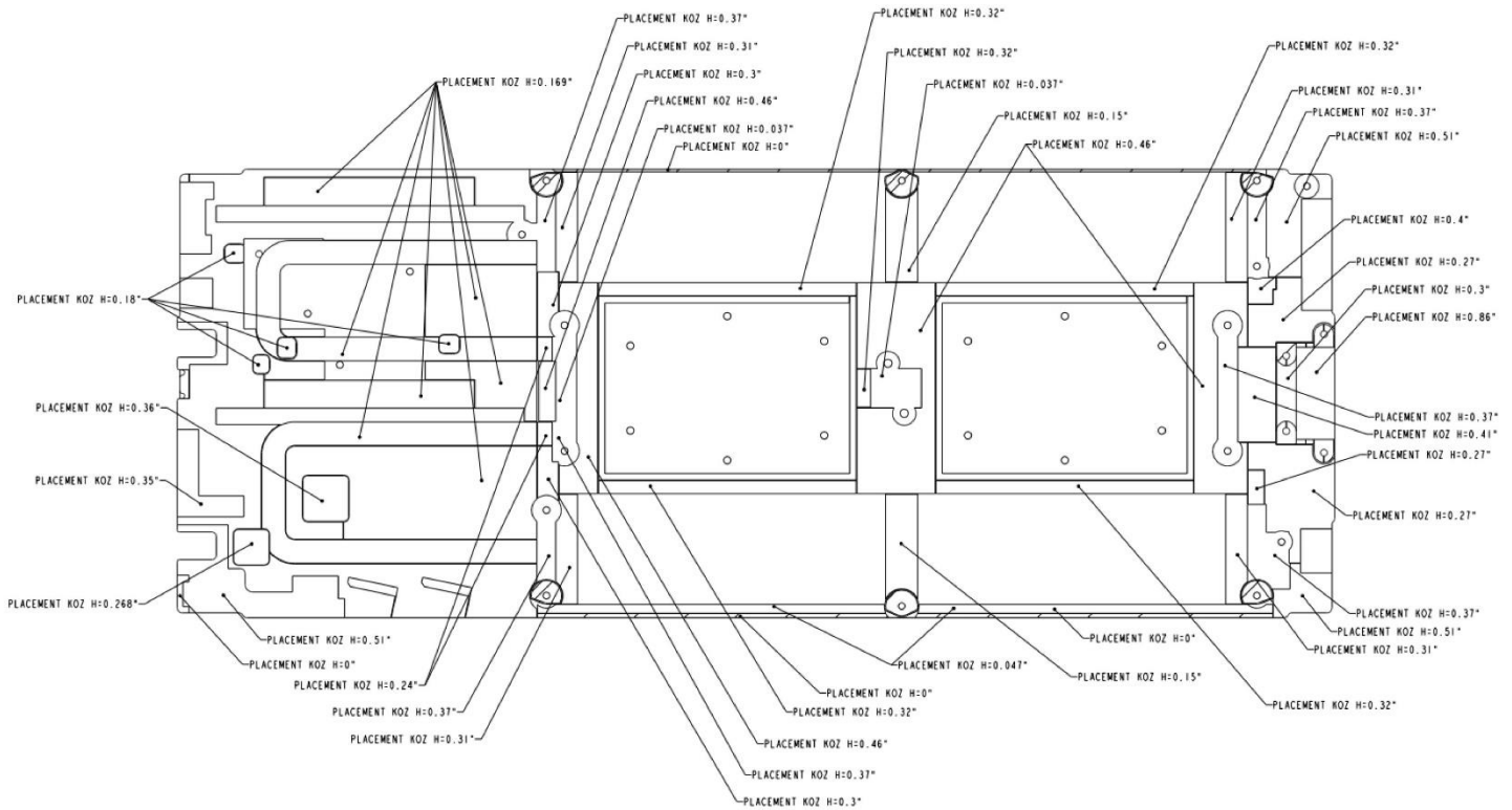
Figure 117. Intel® Server Board D50TNP1SB Top Surface Keep Out Zone
