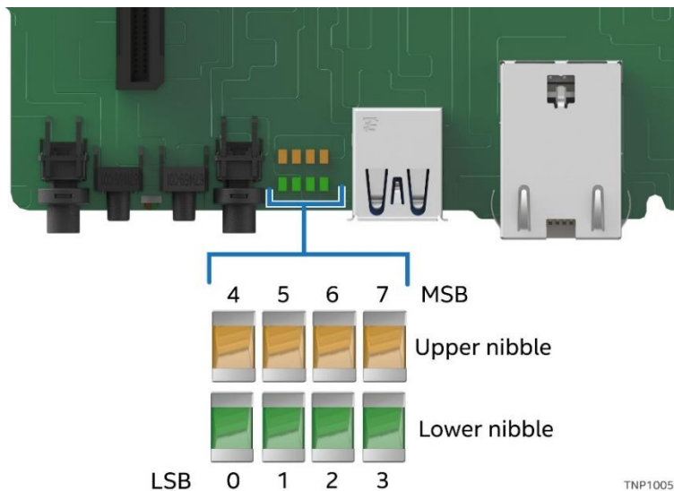
Figure 116. Onboard POST Diagnostic LEDs
