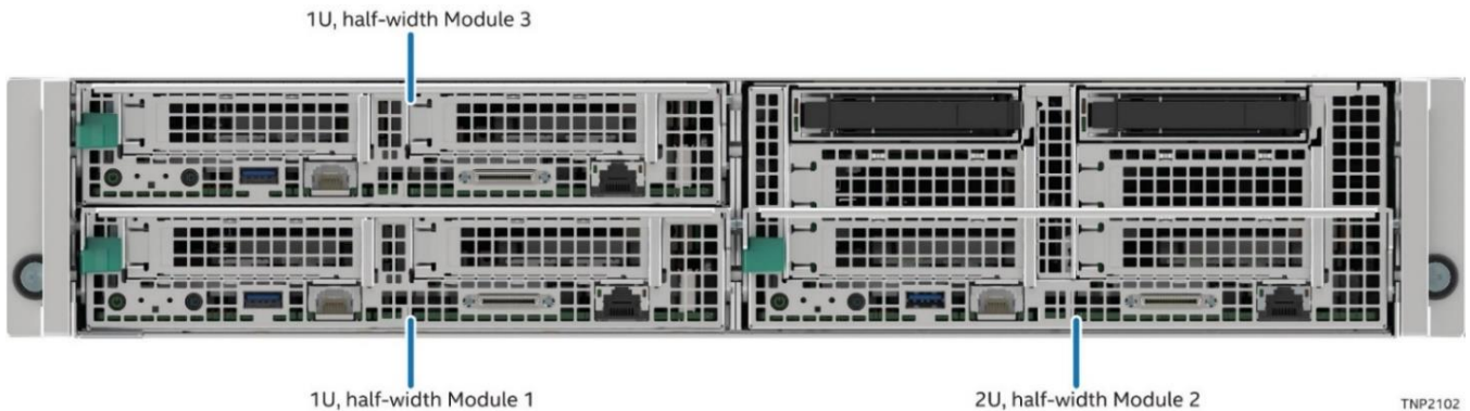
Figure 42. Module Identification for Three-Module System Configuration
