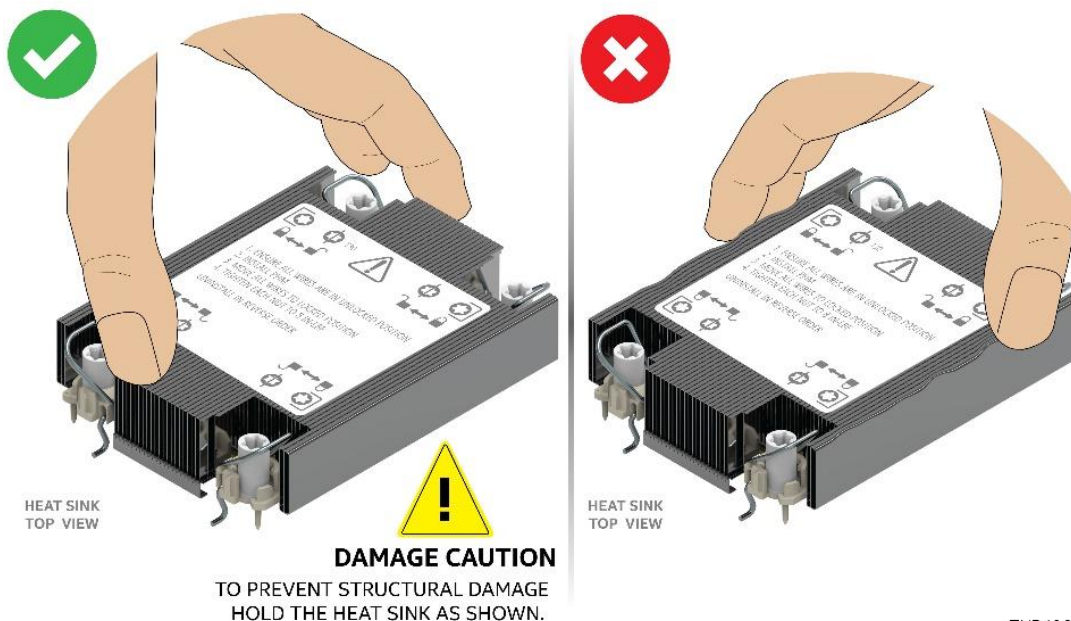
Figure 128. Processor Heat Sink Handling
