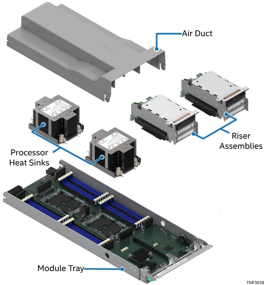
Figure 22. 2U Management Module Components
