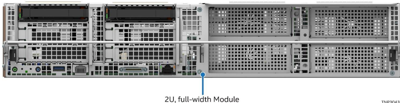
Figure 43. Module Identification for One-Module System Configuration
