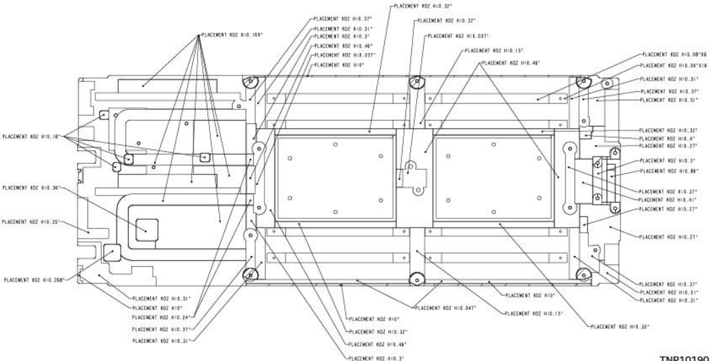
Figure 121. Intel® Server Board D50TNP1SBCR Top Surface Keep Out zone
