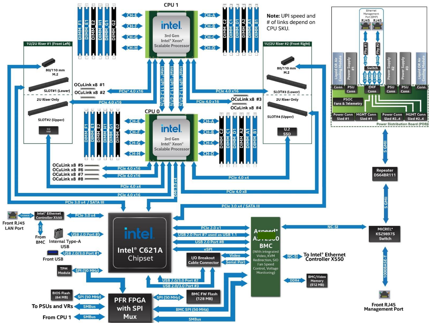
Figure 8. Intel® Server Board D50TNP1SB Architectural Block Diagram
