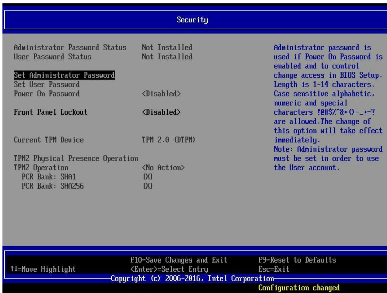
Figure 105. BIOS Setup Security Tab
