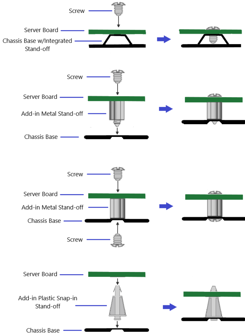
Figure 127. Possible Server Board Mounting Options
