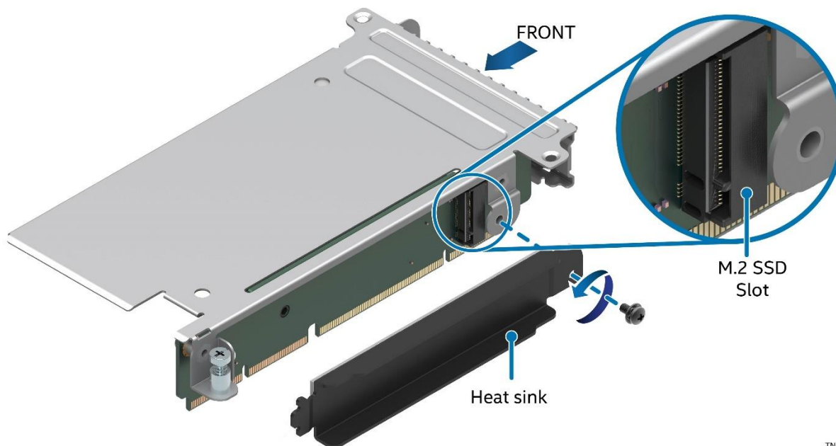
Figure 62. M.2 Slot Location on Riser Card
