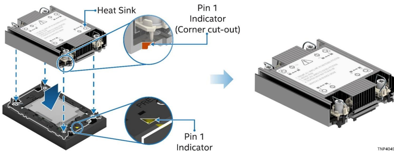
Figure 137. Pin 1 Indicator of Processor Carrier Clip
