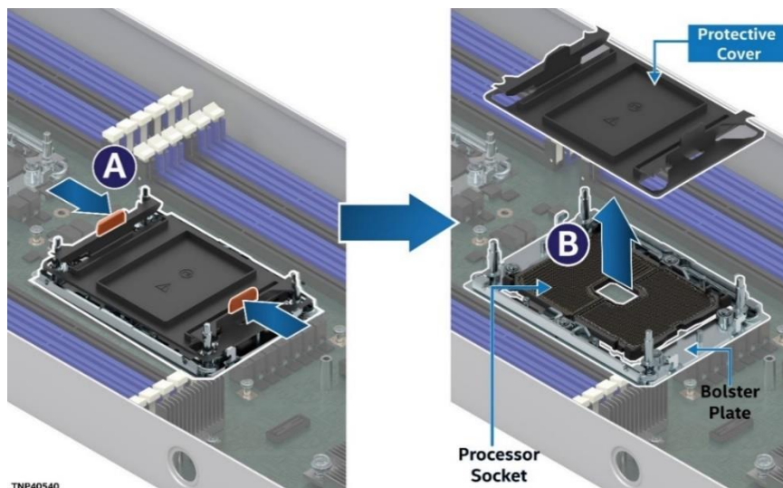
Figure 138. Socket Protective Cover Removal
