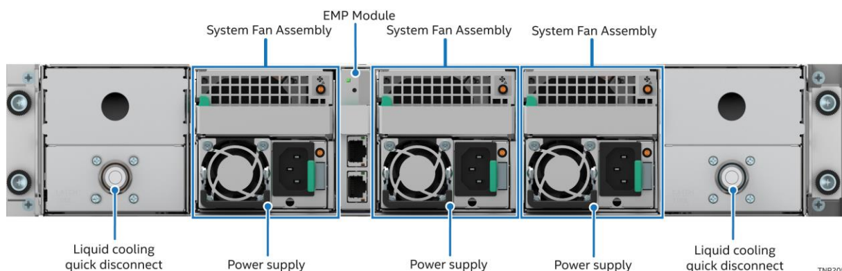
Figure 44. Liquid-Cooled System Back View
