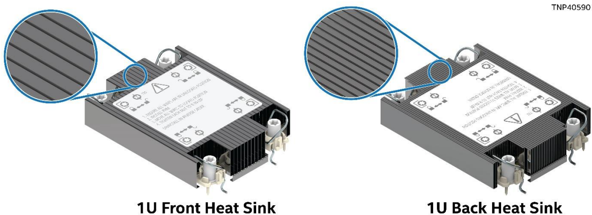
Figure 47. 1U Supported Regular Processor Heat Sinks
