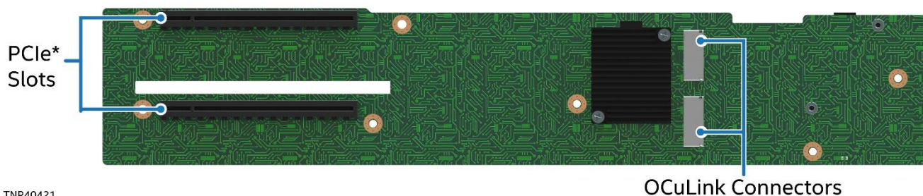
Figure 33. Accelerator Module Riser Card 2 – Front View
