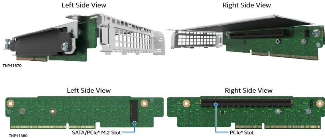
Figure 13. 1U Riser Card Assembly (D50TNP1MHCRCAC, D50TNP1MHCRLC, and D50TNP1MHEVAC)
