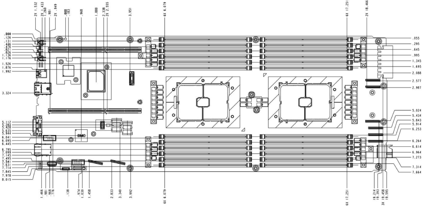
Figure 120. Intel® Server Board D50TNP1SB Holes Position
