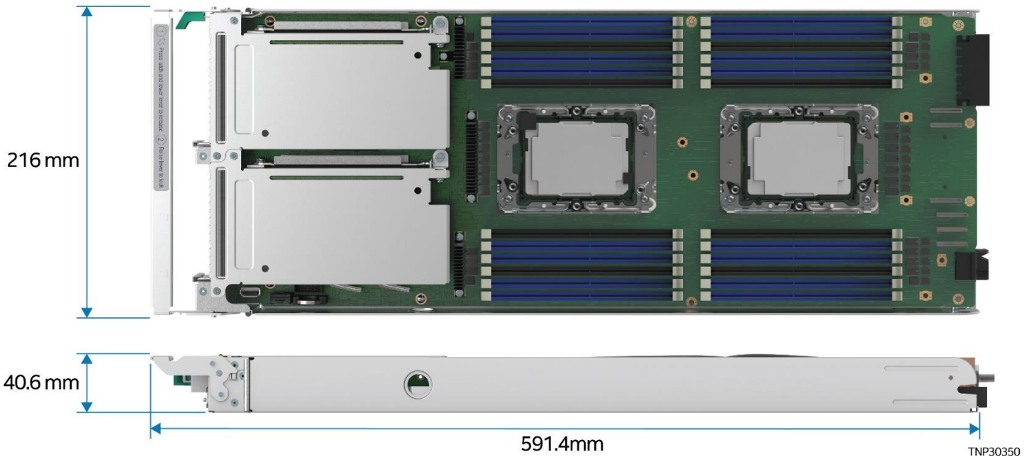
Figure 109. 1U Air-Cooled Compute Module Dimensions
